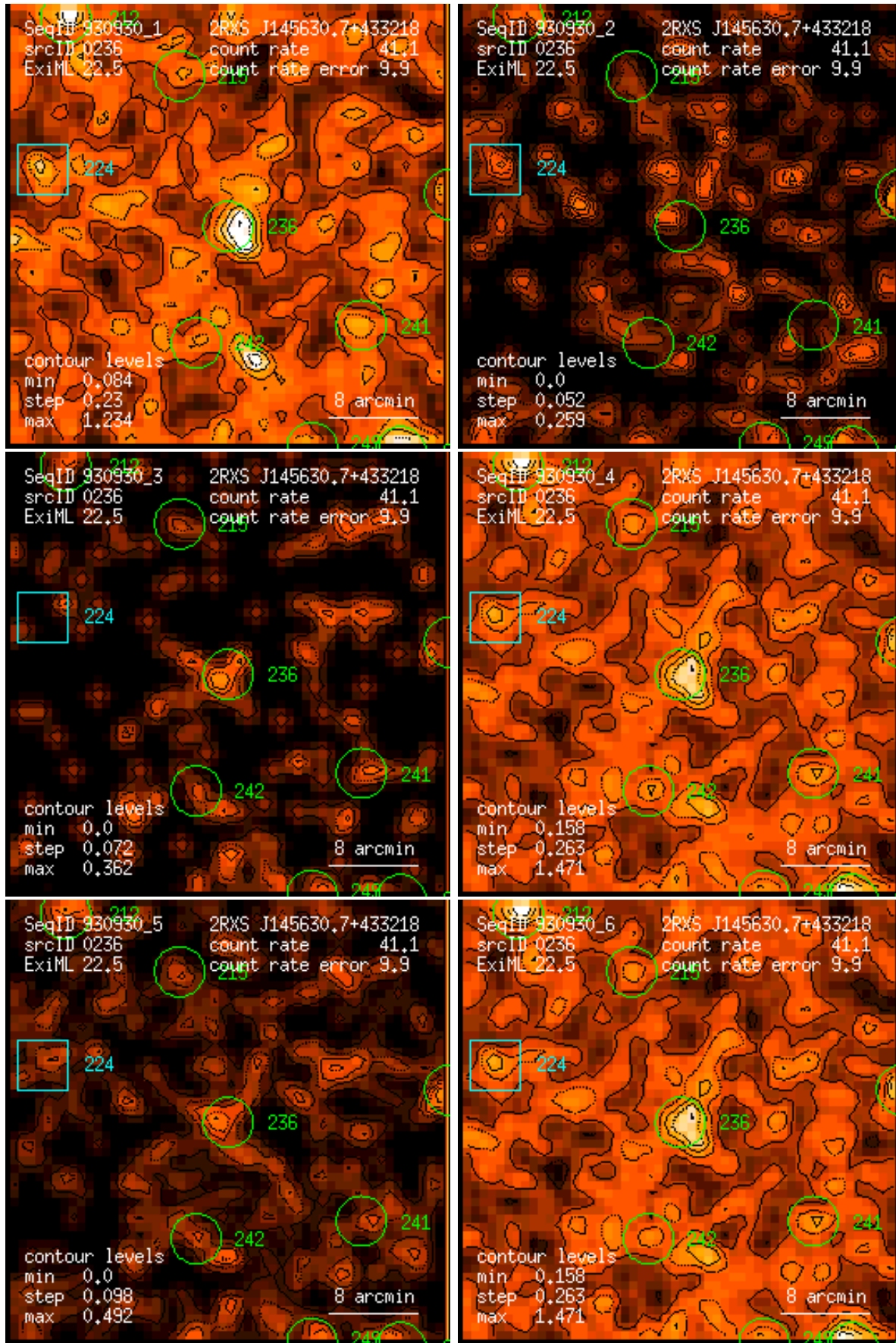
Figure 236: RASS 930930: detection 0236: band rate images, Gaussian filter: (1) PSPC channels 11 – 41, (2) 52 – 90, (3) 91 – 201, (4) 11 – 235, (5) 52 – 201, (6) 11 – 201. Broad band rates in counts/ks. Band rate contour levels in counts/ks/arcmin 2 .
