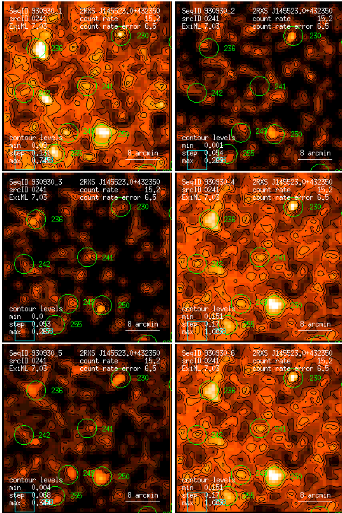
Figure 241: RASS 930930: detection 0241: band rate images, Gaussian filter: (1) PSPC channels 11 – 41, (2) 52 – 90, (3) 91 – 201, (4) 11 – 235, (5) 52 – 201, (6) 11 – 201. Broad band rates in counts/ks. Band rate contour levels in counts/ks/arcmin 2 .
