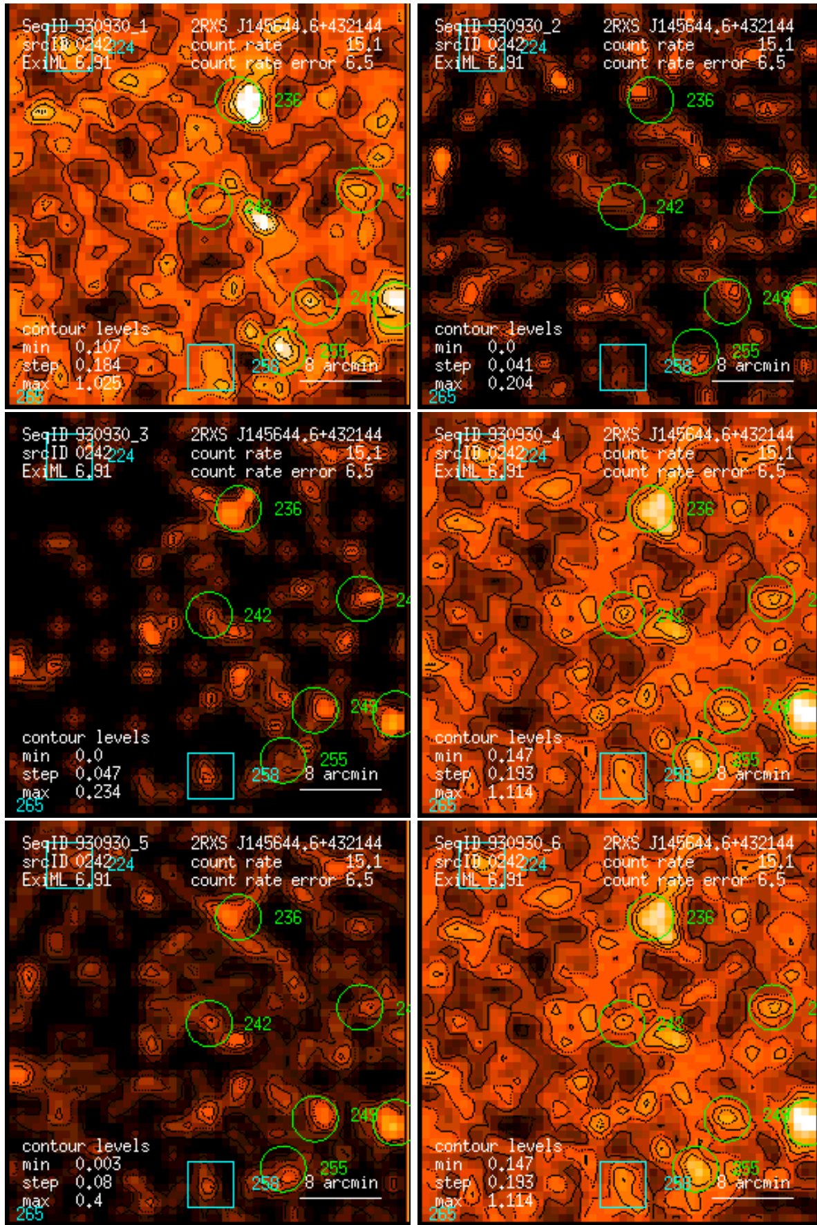
Figure 242: RASS 930930: detection 0242: band rate images, Gaussian filter: (1) PSPC channels 11 – 41, (2) 52 – 90, (3) 91 – 201, (4) 11 – 235, (5) 52 – 201, (6) 11 – 201. Broad band rates in counts/ks. Band rate contour levels in counts/ks/arcmin 2 .
