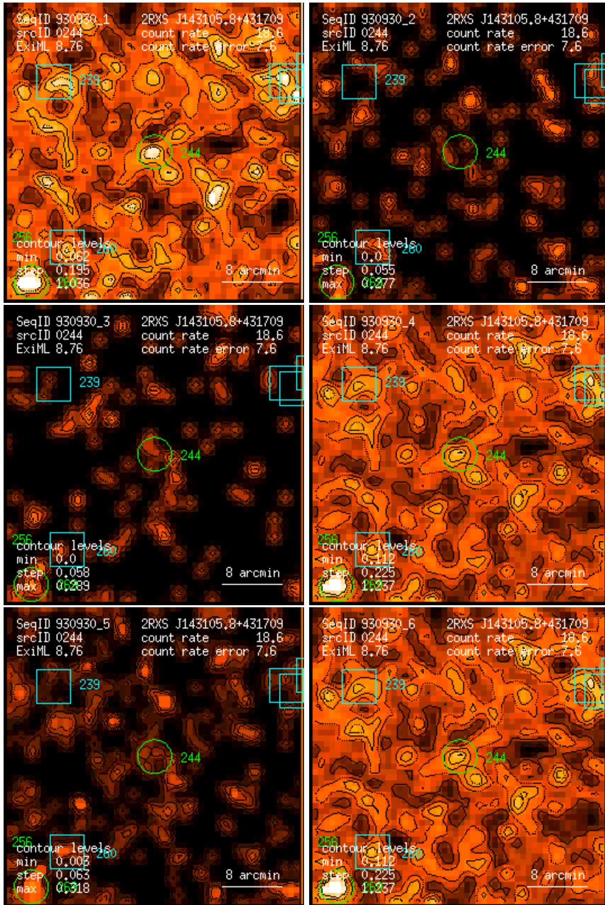
Figure 244: RASS 930930: detection 0244: band rate images, Gaussian filter: (1) PSPC channels 11 – 41, (2) 52 – 90, (3) 91 – 201, (4) 11 – 235, (5) 52 – 201, (6) 11 – 201. Broad band rates in counts/ks. Band rate contour levels in counts/ks/arcmin 2 .
