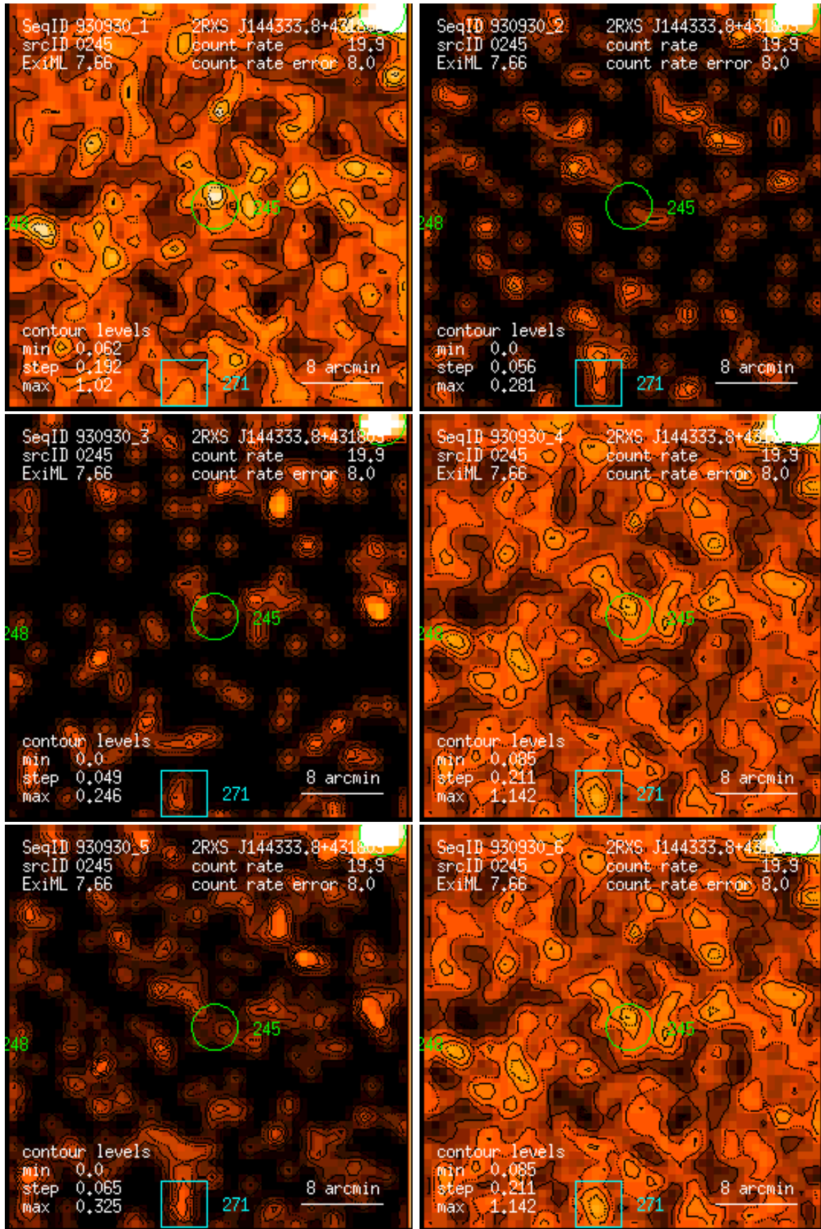
Figure 245: RASS 930930: detection 0245: band rate images, Gaussian filter: (1) PSPC channels 11 – 41, (2) 52 – 90, (3) 91 – 201, (4) 11 – 235, (5) 52 – 201, (6) 11 – 201. Broad band rates in counts/ks. Band rate contour levels in counts/ks/arcmin 2 .
