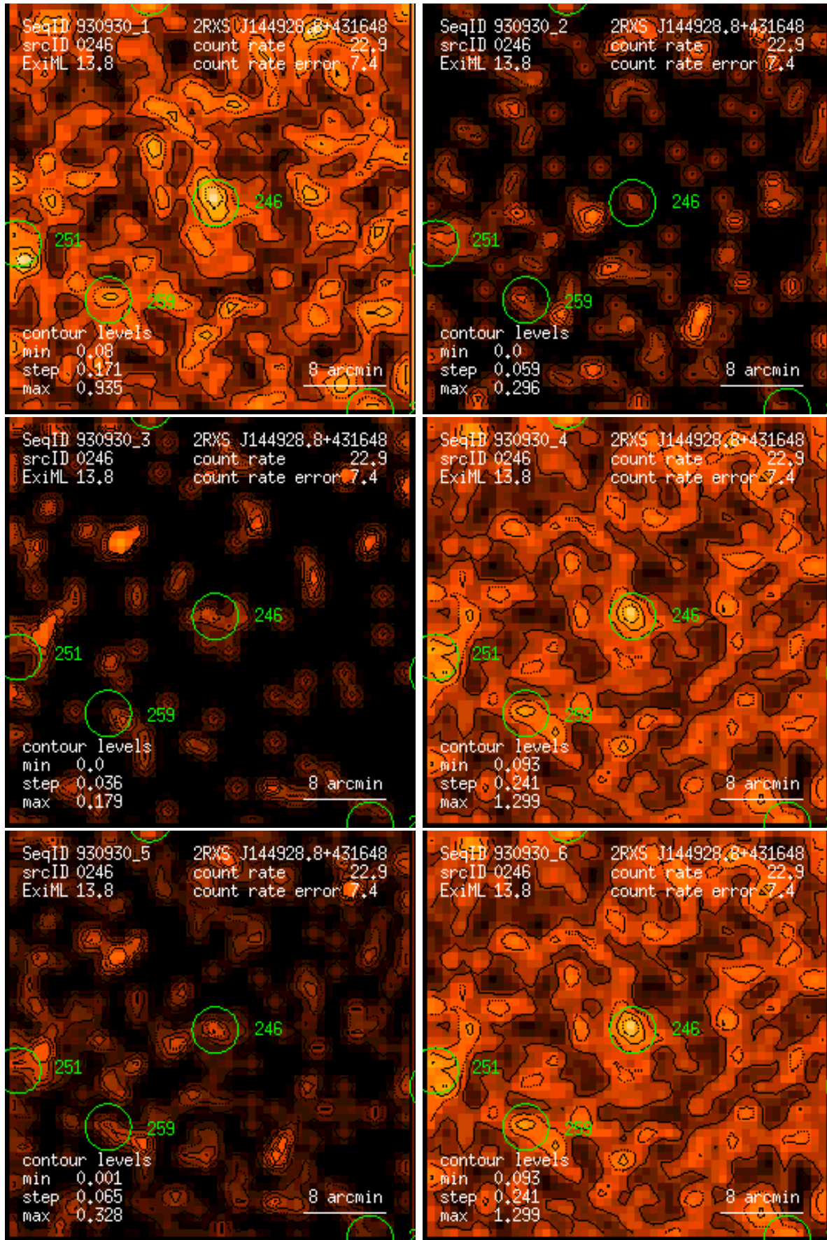
Figure 246: RASS 930930: detection 0246: band rate images, Gaussian filter: (1) PSPC channels 11 – 41, (2) 52 – 90, (3) 91 – 201, (4) 11 – 235, (5) 52 – 201, (6) 11 – 201. Broad band rates in counts/ks. Band rate contour levels in counts/ks/arcmin 2 .
