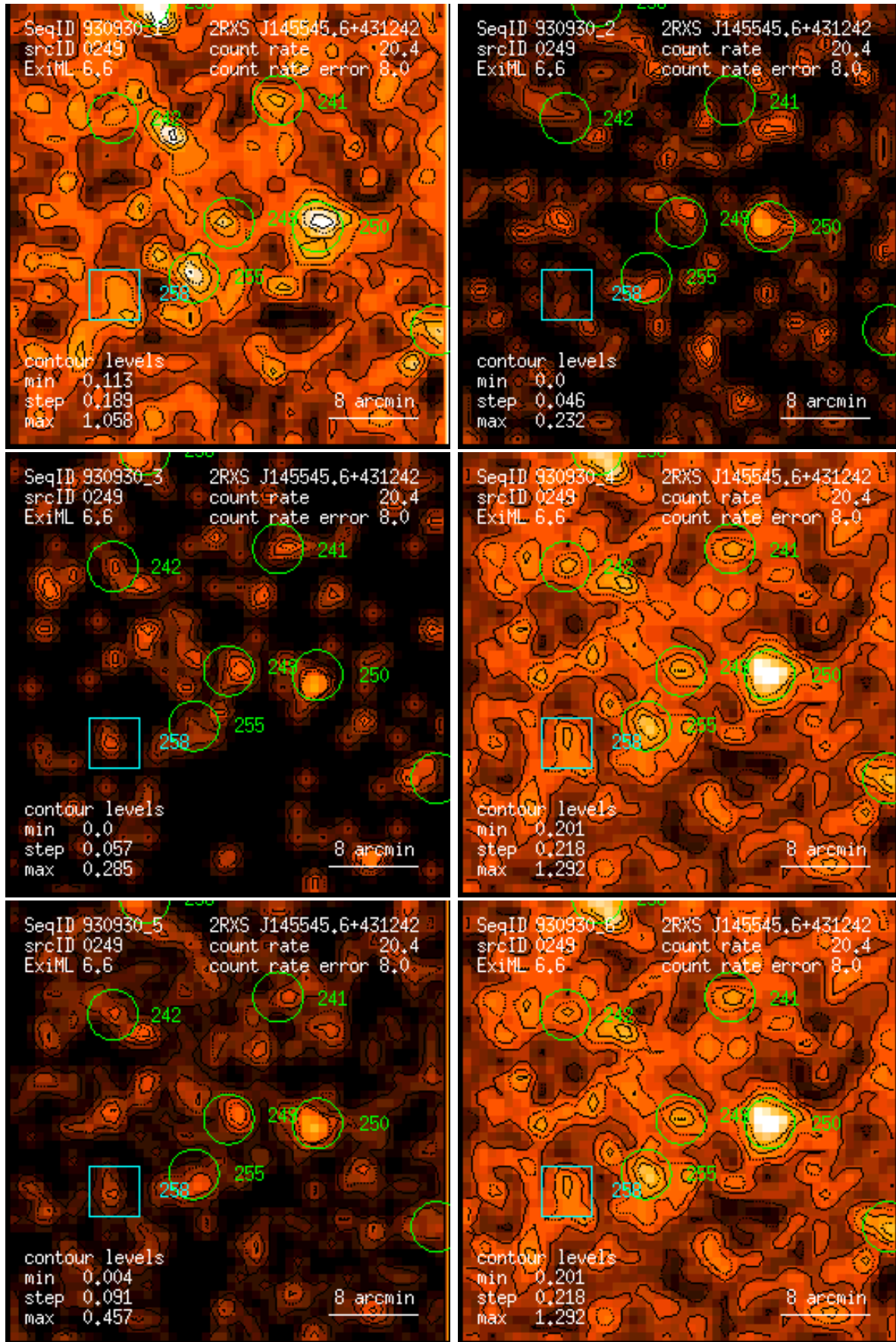
Figure 249: RASS 930930: detection 0249: band rate images, Gaussian filter: (1) PSPC channels 11 – 41, (2) 52 – 90, (3) 91 – 201, (4) 11 – 235, (5) 52 – 201, (6) 11 – 201. Broad band rates in counts/ks. Band rate contour levels in counts/ks/arcmin 2 .
