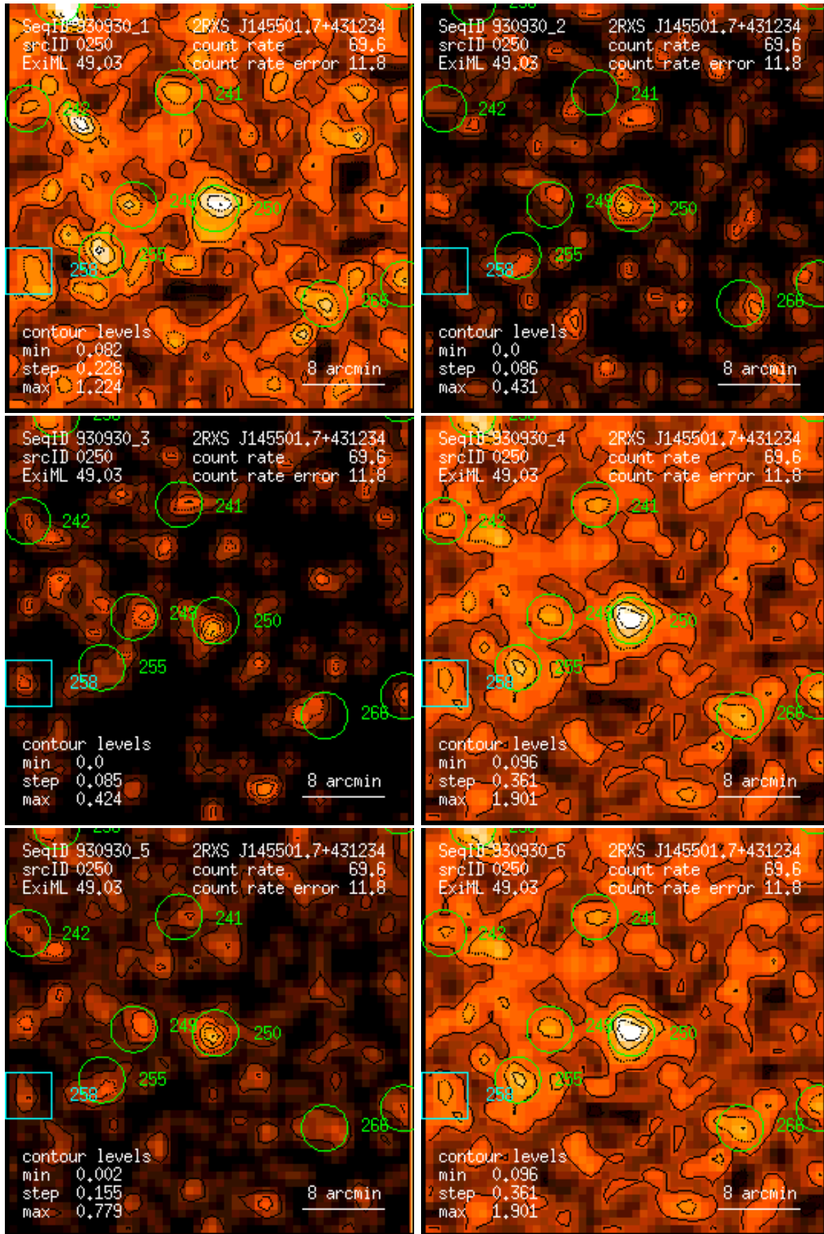
Figure 250: RASS 930930: detection 0250: band rate images, Gaussian filter: (1) PSPC channels 11 – 41, (2) 52 – 90, (3) 91 – 201, (4) 11 – 235, (5) 52 – 201, (6) 11 – 201. Broad band rates in counts/ks. Band rate contour levels in counts/ks/arcmin 2 .
