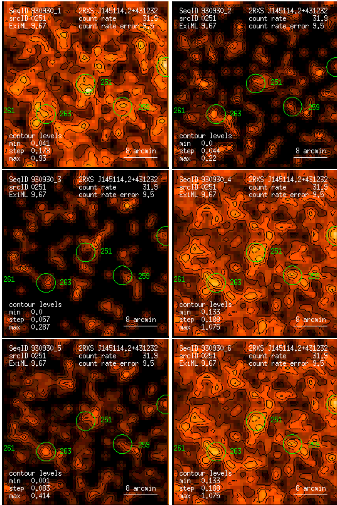
Figure 251: RASS 930930: detection 0251: band rate images, Gaussian filter: (1) PSPC channels 11 – 41, (2) 52 – 90, (3) 91 – 201, (4) 11 – 235, (5) 52 – 201, (6) 11 – 201. Broad band rates in counts/ks. Band rate contour levels in counts/ks/arcmin 2 .
