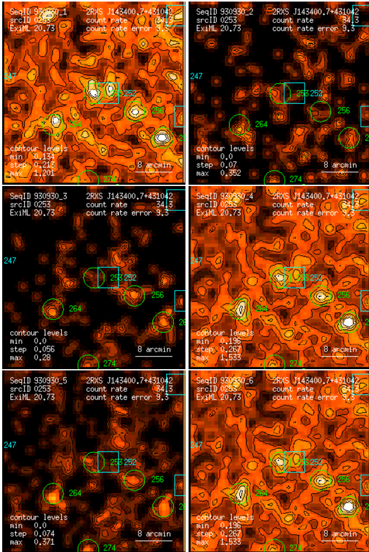
Figure 253: RASS 930930: detection 0253: band rate images, Gaussian filter: (1) PSPC channels 11 – 41, (2) 52 – 90, (3) 91 – 201, (4) 11 – 235, (5) 52 – 201, (6) 11 – 201. Broad band rates in counts/ks. Band rate contour levels in counts/ks/arcmin 2 .
