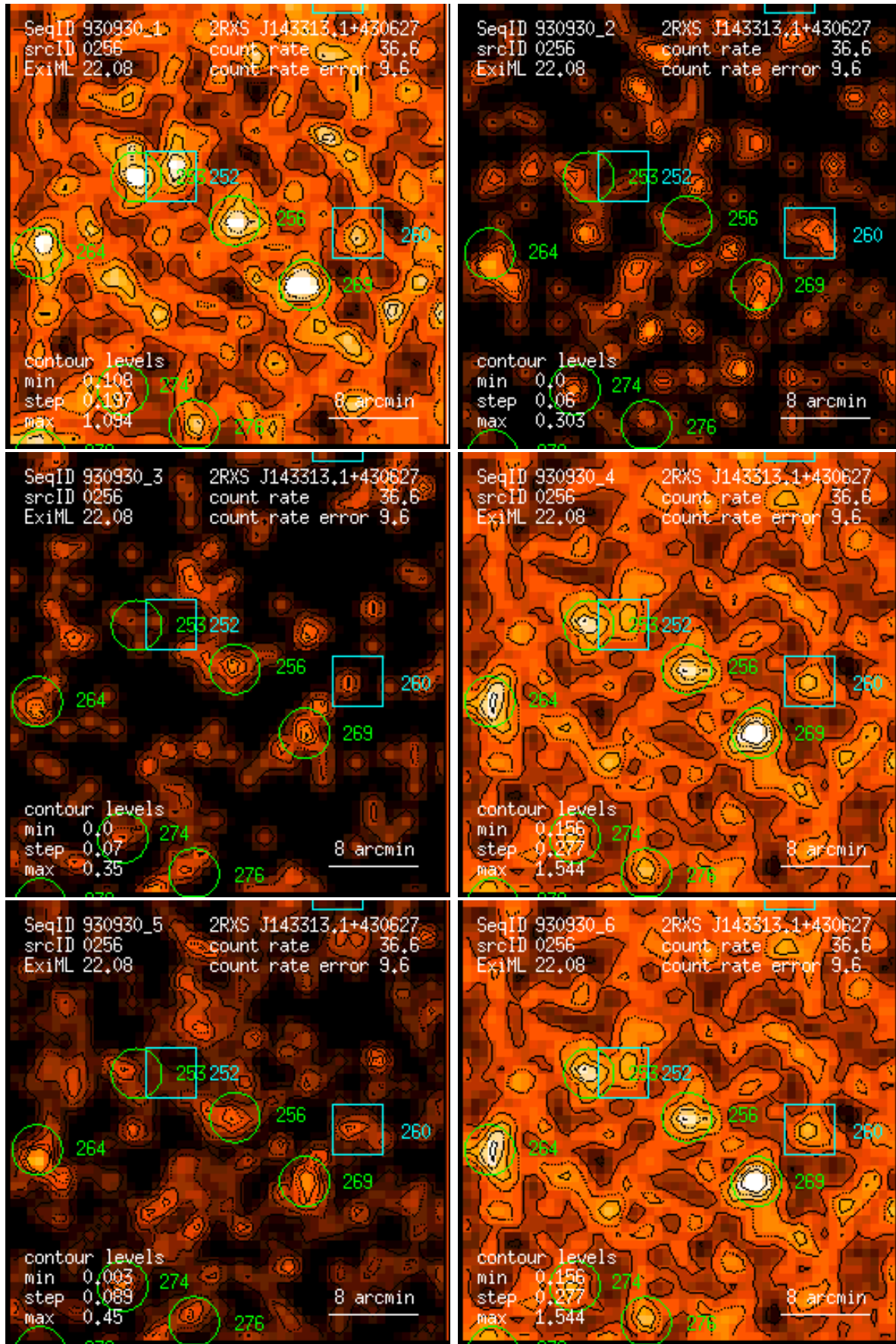
Figure 256: RASS 930930: detection 0256: band rate images, Gaussian filter: (1) PSPC channels 11 – 41, (2) 52 – 90, (3) 91 – 201, (4) 11 – 235, (5) 52 – 201, (6) 11 – 201. Broad band rates in counts/ks. Band rate contour levels in counts/ks/arcmin 2 .
