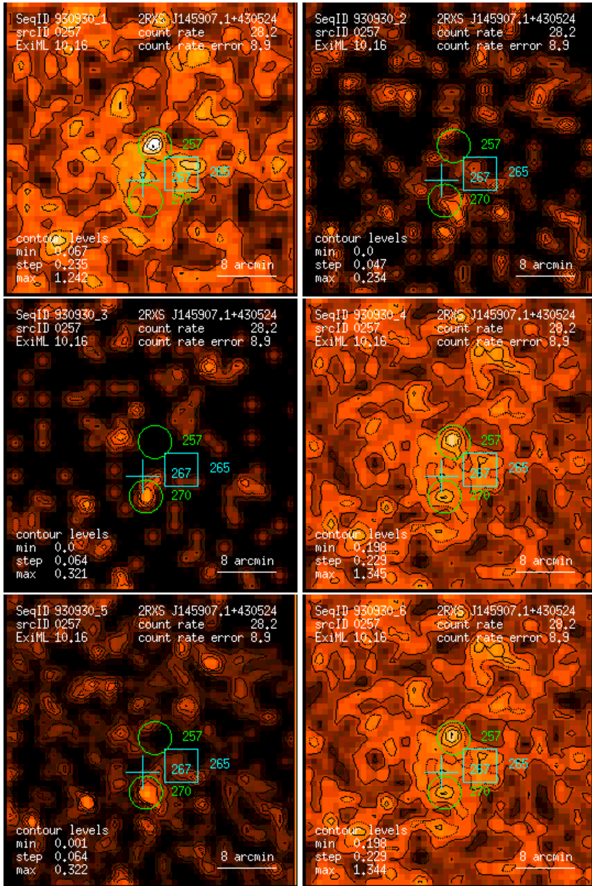
Figure 257: RASS 930930: detection 0257: band rate images, Gaussian filter: (1) PSPC channels 11 – 41, (2) 52 – 90, (3) 91 – 201, (4) 11 – 235, (5) 52 – 201, (6) 11 – 201. Broad band rates in counts/ks. Band rate contour levels in counts/ks/arcmin 2 .
