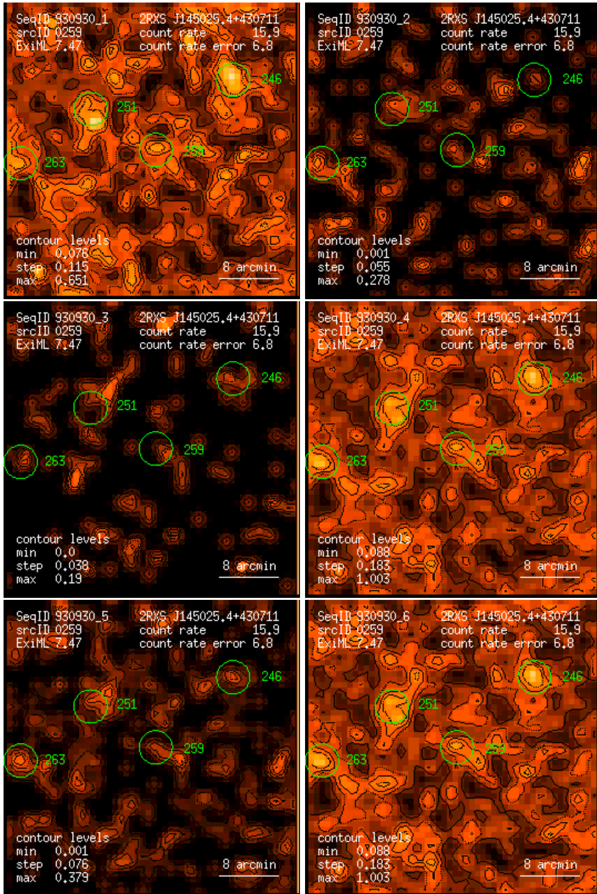
Figure 259: RASS 930930: detection 0259: band rate images, Gaussian filter: (1) PSPC channels 11 – 41, (2) 52 – 90, (3) 91 – 201, (4) 11 – 235, (5) 52 – 201, (6) 11 – 201. Broad band rates in counts/ks. Band rate contour levels in counts/ks/arcmin 2 .
