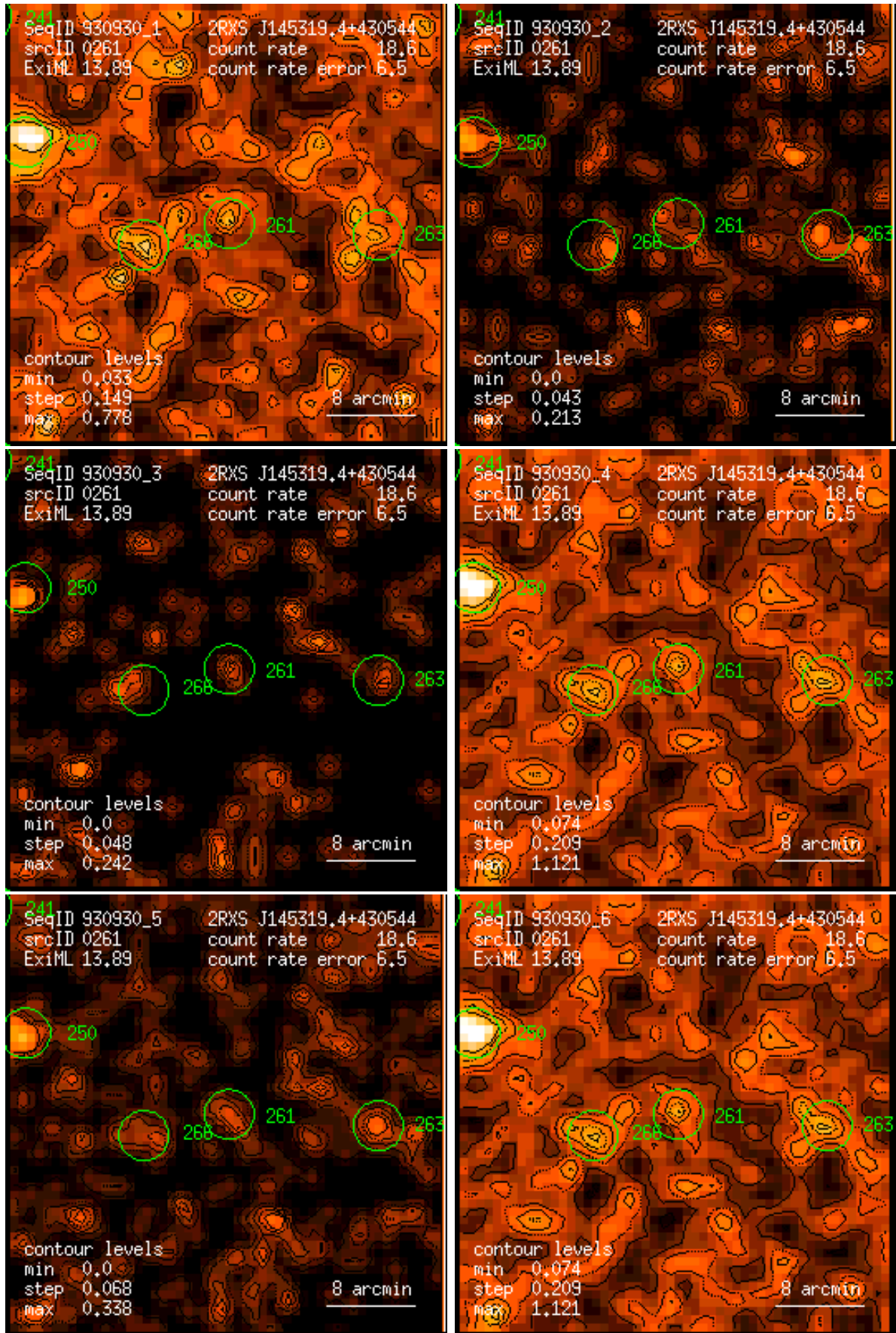
Figure 261: RASS 930930: detection 0261: band rate images, Gaussian filter: (1) PSPC channels 11 – 41, (2) 52 – 90, (3) 91 – 201, (4) 11 – 235, (5) 52 – 201, (6) 11 – 201. Broad band rates in counts/ks. Band rate contour levels in counts/ks/arcmin 2 .
