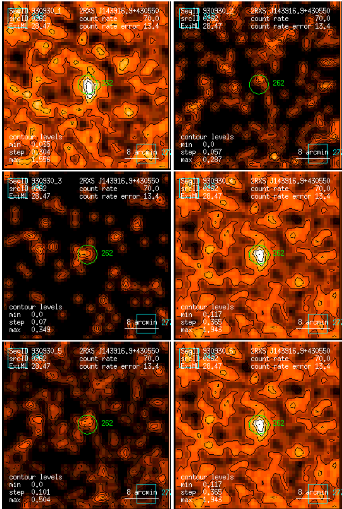
Figure 262: RASS 930930: detection 0262: band rate images, Gaussian filter: (1) PSPC channels 11 – 41, (2) 52 – 90, (3) 91 – 201, (4) 11 – 235, (5) 52 – 201, (6) 11 – 201. Broad band rates in counts/ks. Band rate contour levels in counts/ks/arcmin 2 .
