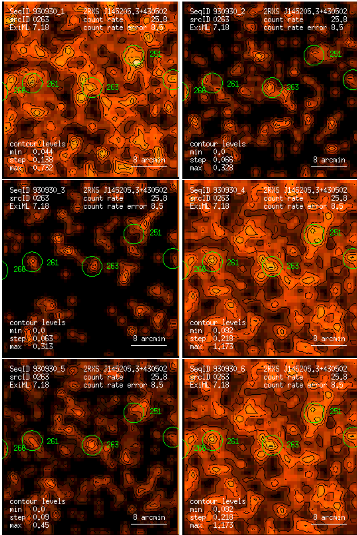
Figure 263: RASS 930930: detection 0263: band rate images, Gaussian filter: (1) PSPC channels 11 – 41, (2) 52 – 90, (3) 91 – 201, (4) 11 – 235, (5) 52 – 201, (6) 11 – 201. Broad band rates in counts/ks. Band rate contour levels in counts/ks/arcmin 2 .
