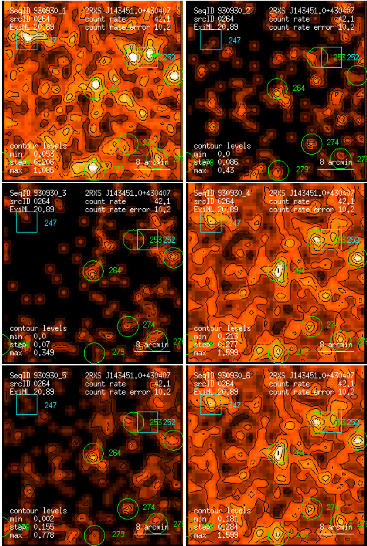
Figure 264: RASS 930930: detection 0264: band rate images, Gaussian filter: (1) PSPC channels 11 – 41, (2) 52 – 90, (3) 91 – 201, (4) 11 – 235, (5) 52 – 201, (6) 11 – 201. Broad band rates in counts/ks. Band rate contour levels in counts/ks/arcmin 2 .
