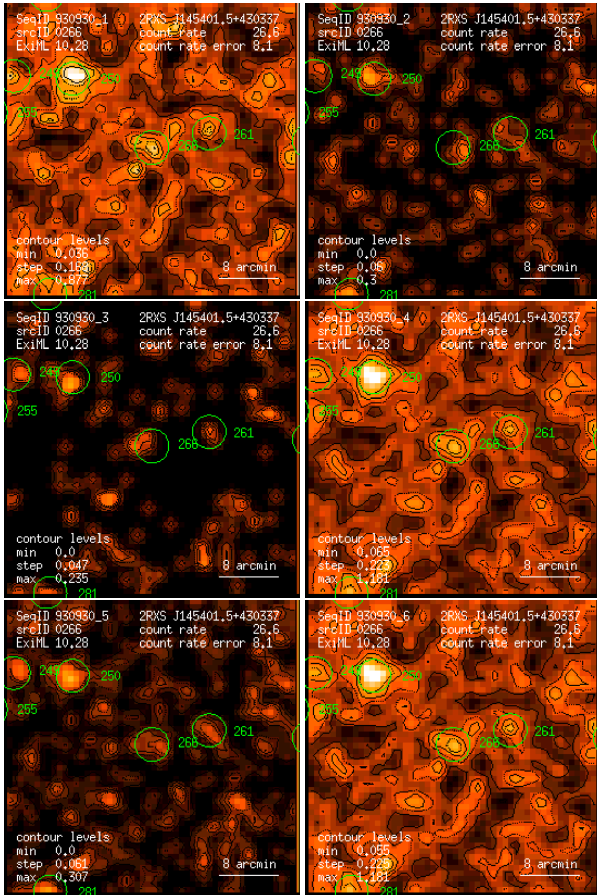
Figure 266: RASS 930930: detection 0266: band rate images, Gaussian filter: (1) PSPC channels 11 – 41, (2) 52 – 90, (3) 91 – 201, (4) 11 – 235, (5) 52 – 201, (6) 11 – 201. Broad band rates in counts/ks. Band rate contour levels in counts/ks/arcmin 2 .
