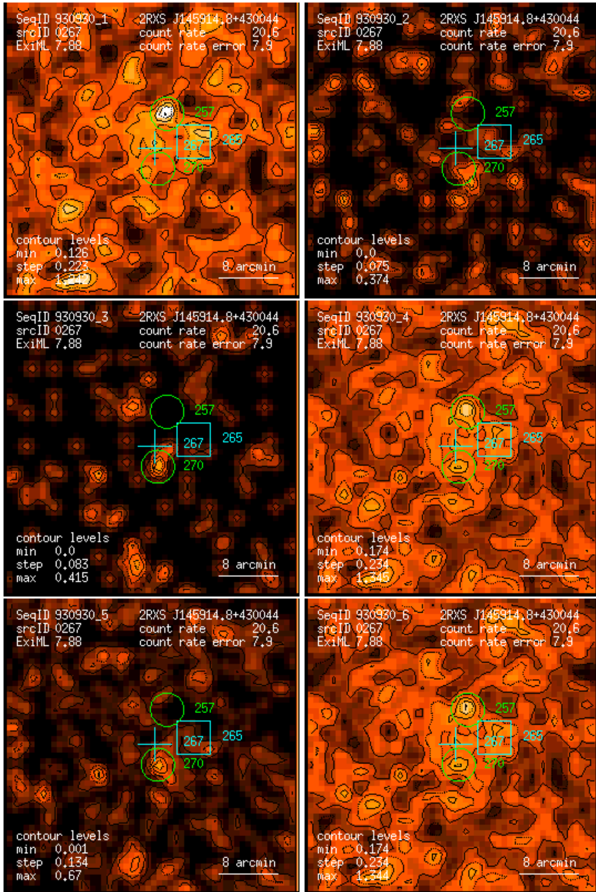
Figure 267: RASS 930930: detection 0267: band rate images, Gaussian filter: (1) PSPC channels 11 – 41, (2) 52 – 90, (3) 91 – 201, (4) 11 – 235, (5) 52 – 201, (6) 11 – 201. Broad band rates in counts/ks. Band rate contour levels in counts/ks/arcmin 2 .
