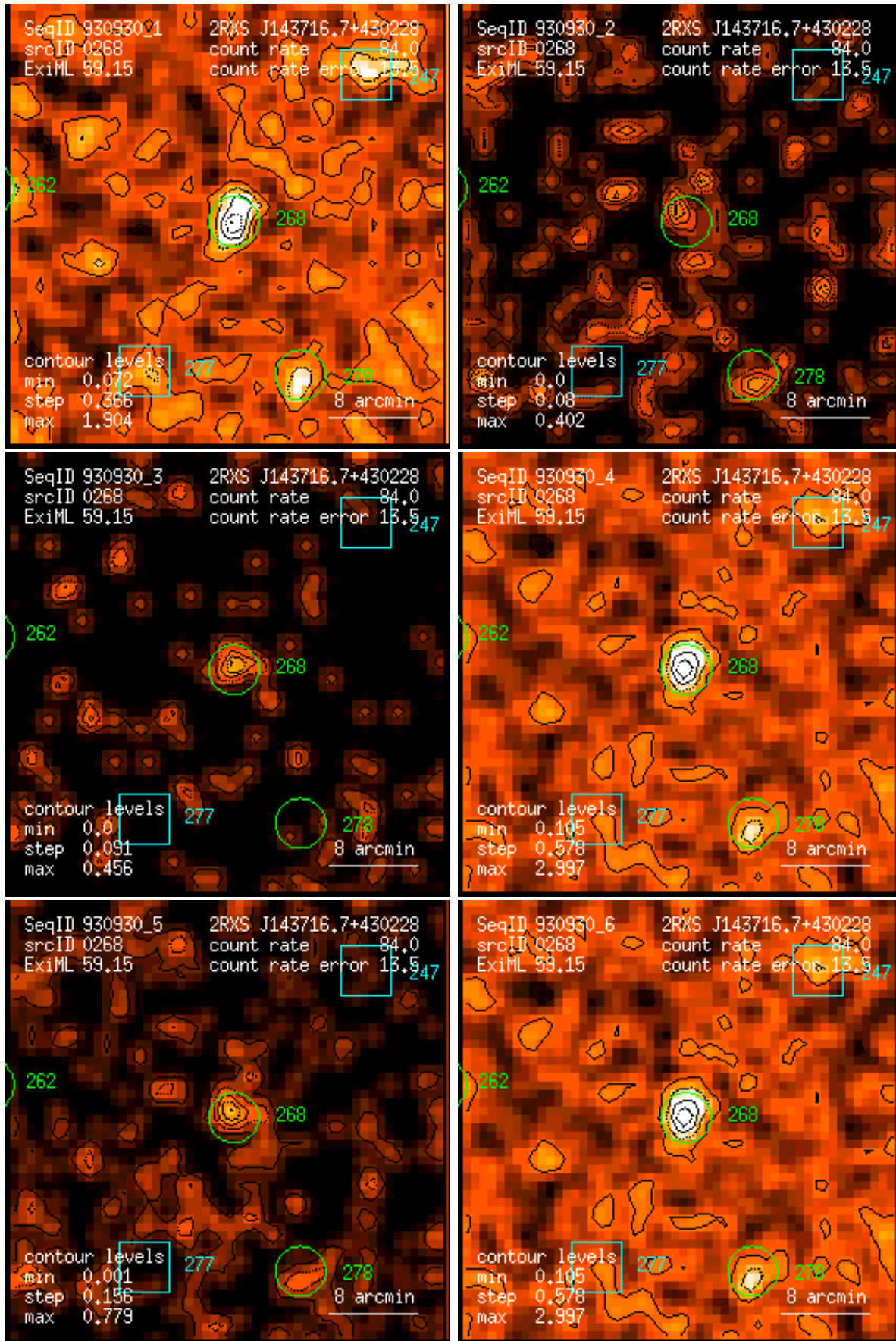
Figure 268: RASS 930930: detection 0268: band rate images, Gaussian filter: (1) PSPC channels 11 – 41, (2) 52 – 90, (3) 91 – 201, (4) 11 – 235, (5) 52 – 201, (6) 11 – 201. Broad band rates in counts/ks. Band rate contour levels in counts/ks/arcmin 2 .
