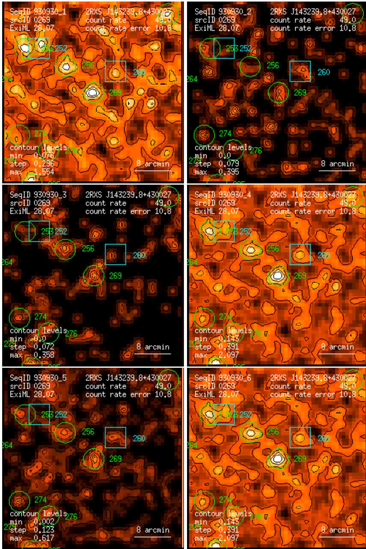
Figure 269: RASS 930930: detection 0269: band rate images, Gaussian filter: (1) PSPC channels 11 – 41, (2) 52 – 90, (3) 91 – 201, (4) 11 – 235, (5) 52 – 201, (6) 11 – 201. Broad band rates in counts/ks. Band rate contour levels in counts/ks/arcmin 2 .
