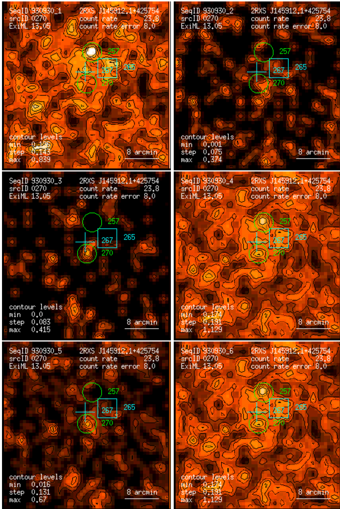
Figure 270: RASS 930930: detection 0270: band rate images, Gaussian filter: (1) PSPC channels 11 – 41, (2) 52 – 90, (3) 91 – 201, (4) 11 – 235, (5) 52 – 201, (6) 11 – 201. Broad band rates in counts/ks. Band rate contour levels in counts/ks/arcmin 2 .
