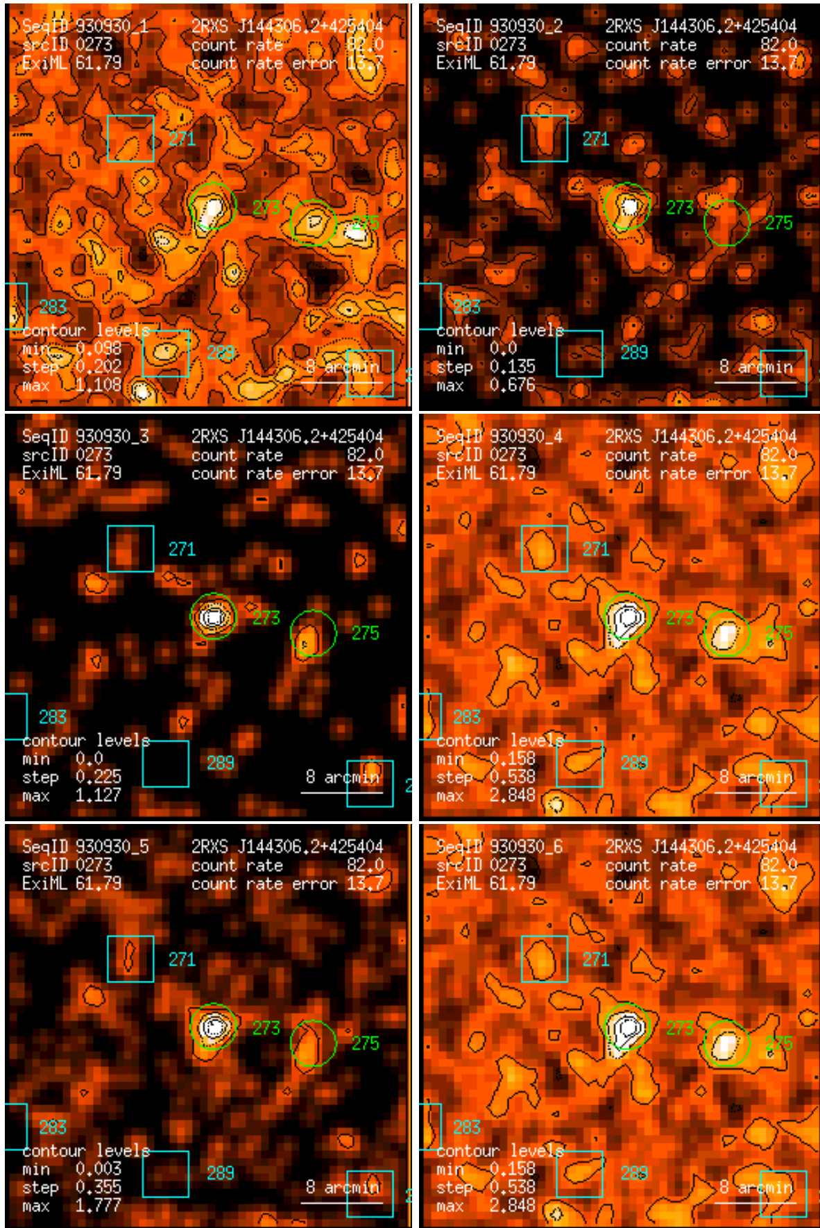
Figure 273: RASS 930930: detection 0273: band rate images, Gaussian filter: (1) PSPC channels 11 – 41, (2) 52 – 90, (3) 91 – 201, (4) 11 – 235, (5) 52 – 201, (6) 11 – 201. Broad band rates in counts/ks. Band rate contour levels in counts/ks/arcmin 2 .
