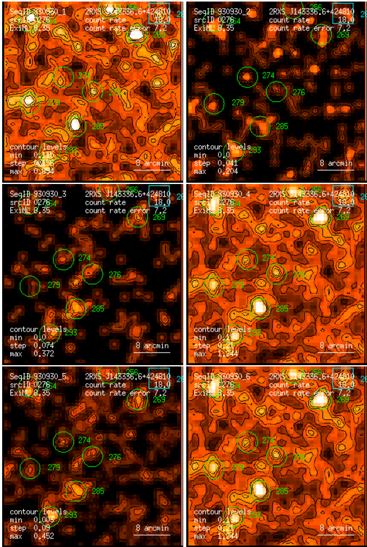
Figure 276: RASS 930930: detection 0276: band rate images, Gaussian filter: (1) PSPC channels 11 – 41, (2) 52 – 90, (3) 91 – 201, (4) 11 – 235, (5) 52 – 201, (6) 11 – 201. Broad band rates in counts/ks. Band rate contour levels in counts/ks/arcmin 2 .
