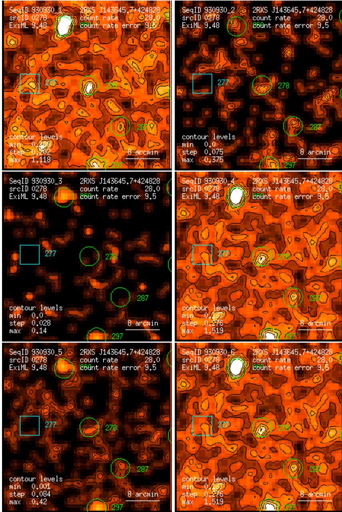
Figure 278: RASS 930930: detection 0278: band rate images, Gaussian filter: (1) PSPC channels 11 – 41, (2) 52 – 90, (3) 91 – 201, (4) 11 – 235, (5) 52 – 201, (6) 11 – 201. Broad band rates in counts/ks. Band rate contour levels in counts/ks/arcmin 2 .
