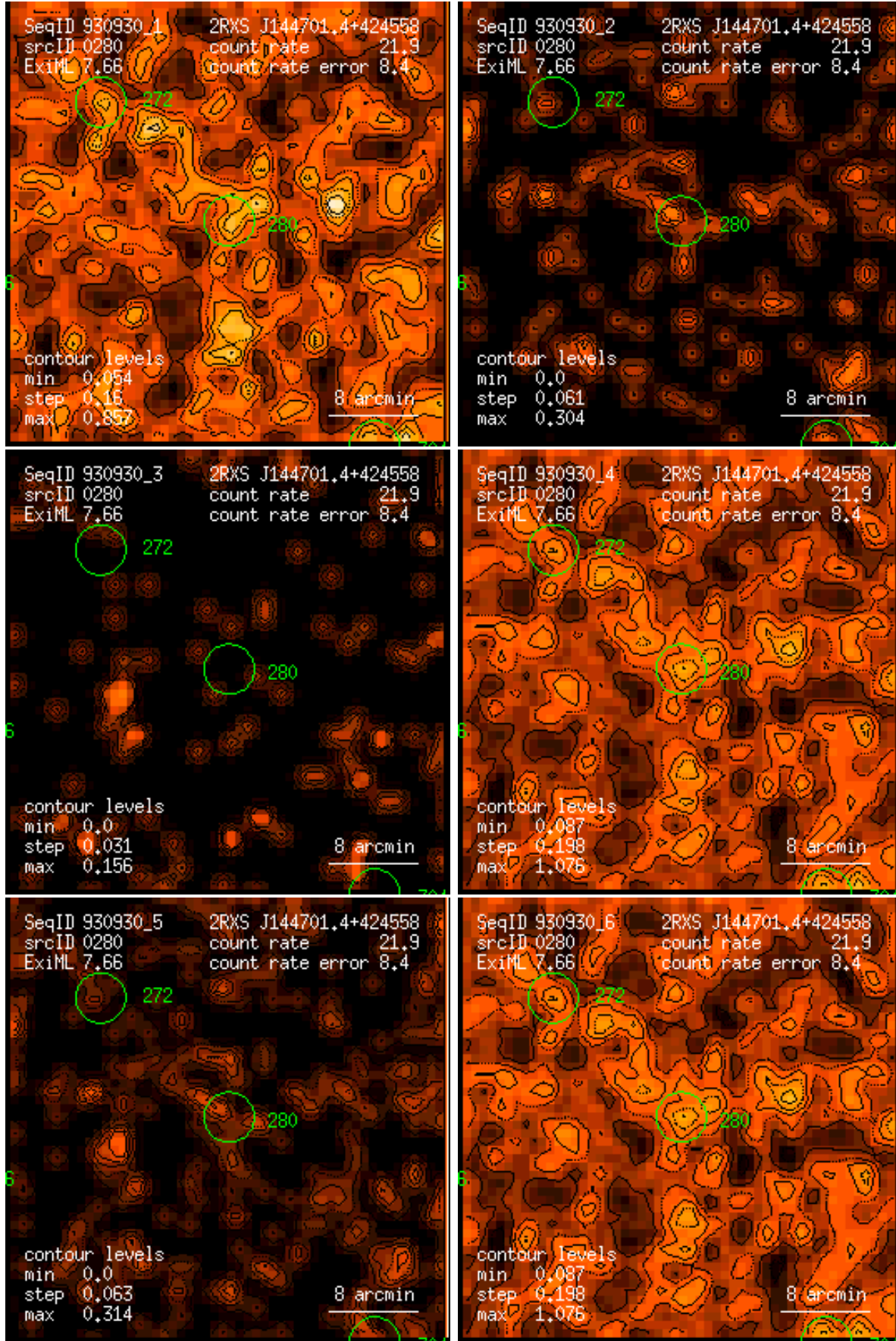
Figure 280: RASS 930930: detection 0280: band rate images, Gaussian filter: (1) PSPC channels 11 – 41, (2) 52 – 90, (3) 91 – 201, (4) 11 – 235, (5) 52 – 201, (6) 11 – 201. Broad band rates in counts/ks. Band rate contour levels in counts/ks/arcmin 2 .
