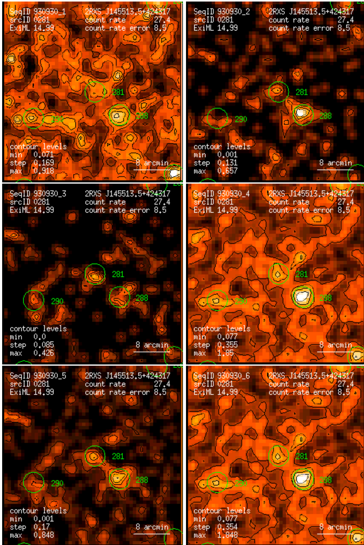
Figure 281: RASS 930930: detection 0281: band rate images, Gaussian filter: (1) PSPC channels 11 – 41, (2) 52 – 90, (3) 91 – 201, (4) 11 – 235, (5) 52 – 201, (6) 11 – 201. Broad band rates in counts/ks. Band rate contour levels in counts/ks/arcmin 2 .
