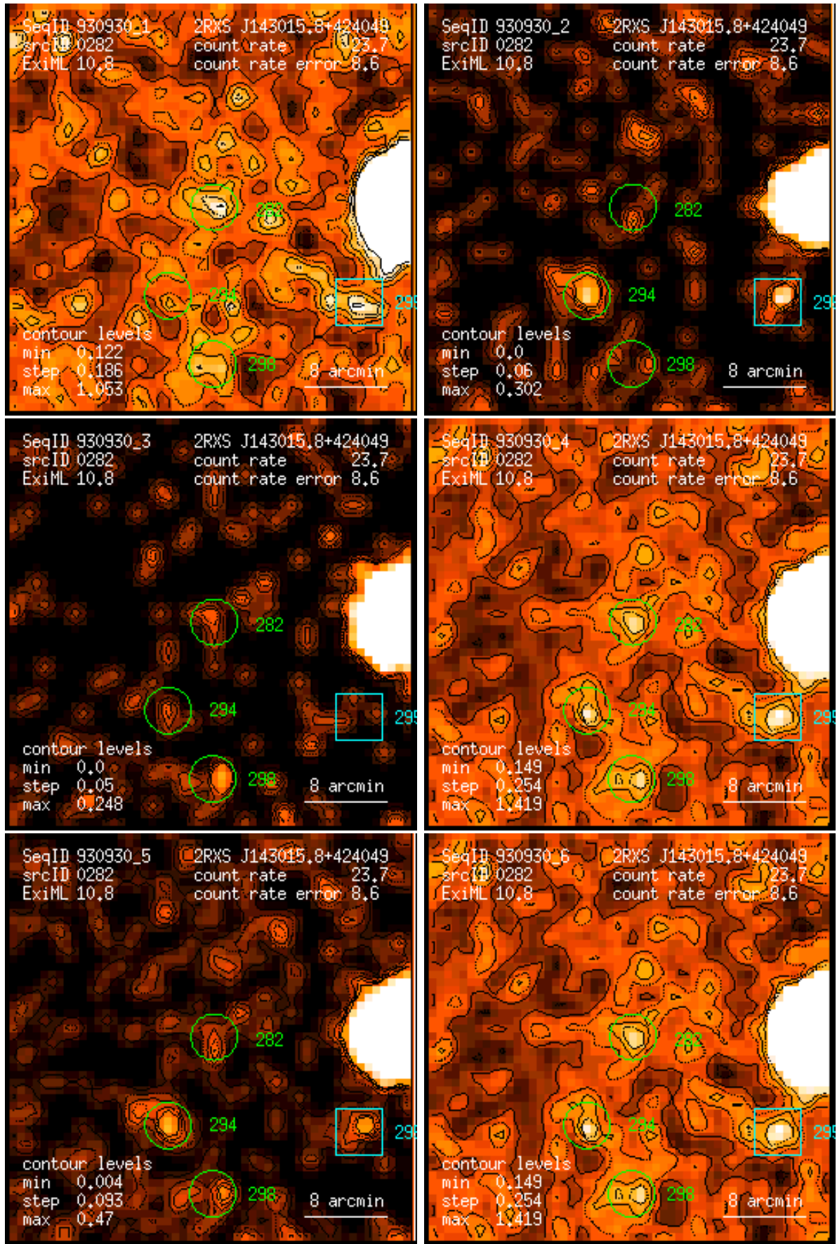
Figure 282: RASS 930930: detection 0282: band rate images, Gaussian filter: (1) PSPC channels 11 – 41, (2) 52 – 90, (3) 91 – 201, (4) 11 – 235, (5) 52 – 201, (6) 11 – 201. Broad band rates in counts/ks. Band rate contour levels in counts/ks/arcmin 2 .
