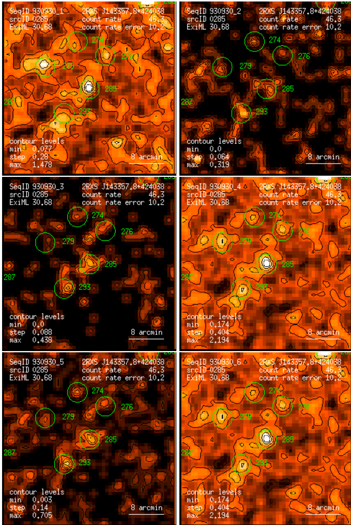
Figure 285: RASS 930930: detection 0285: band rate images, Gaussian filter: (1) PSPC channels 11 – 41, (2) 52 – 90, (3) 91 – 201, (4) 11 – 235, (5) 52 – 201, (6) 11 – 201. Broad band rates in counts/ks. Band rate contour levels in counts/ks/arcmin 2 .
