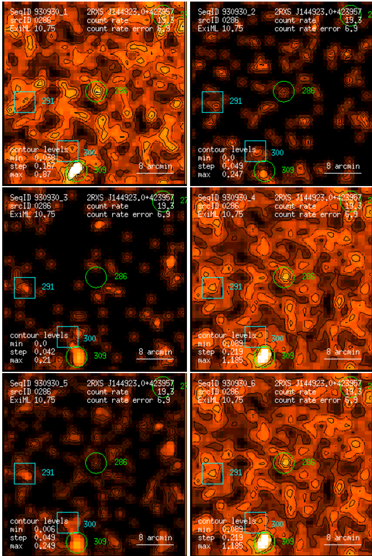
Figure 286: RASS 930930: detection 0286: band rate images, Gaussian filter: (1) PSPC channels 11 – 41, (2) 52 – 90, (3) 91 – 201, (4) 11 – 235, (5) 52 – 201, (6) 11 – 201. Broad band rates in counts/ks. Band rate contour levels in counts/ks/arcmin 2 .
