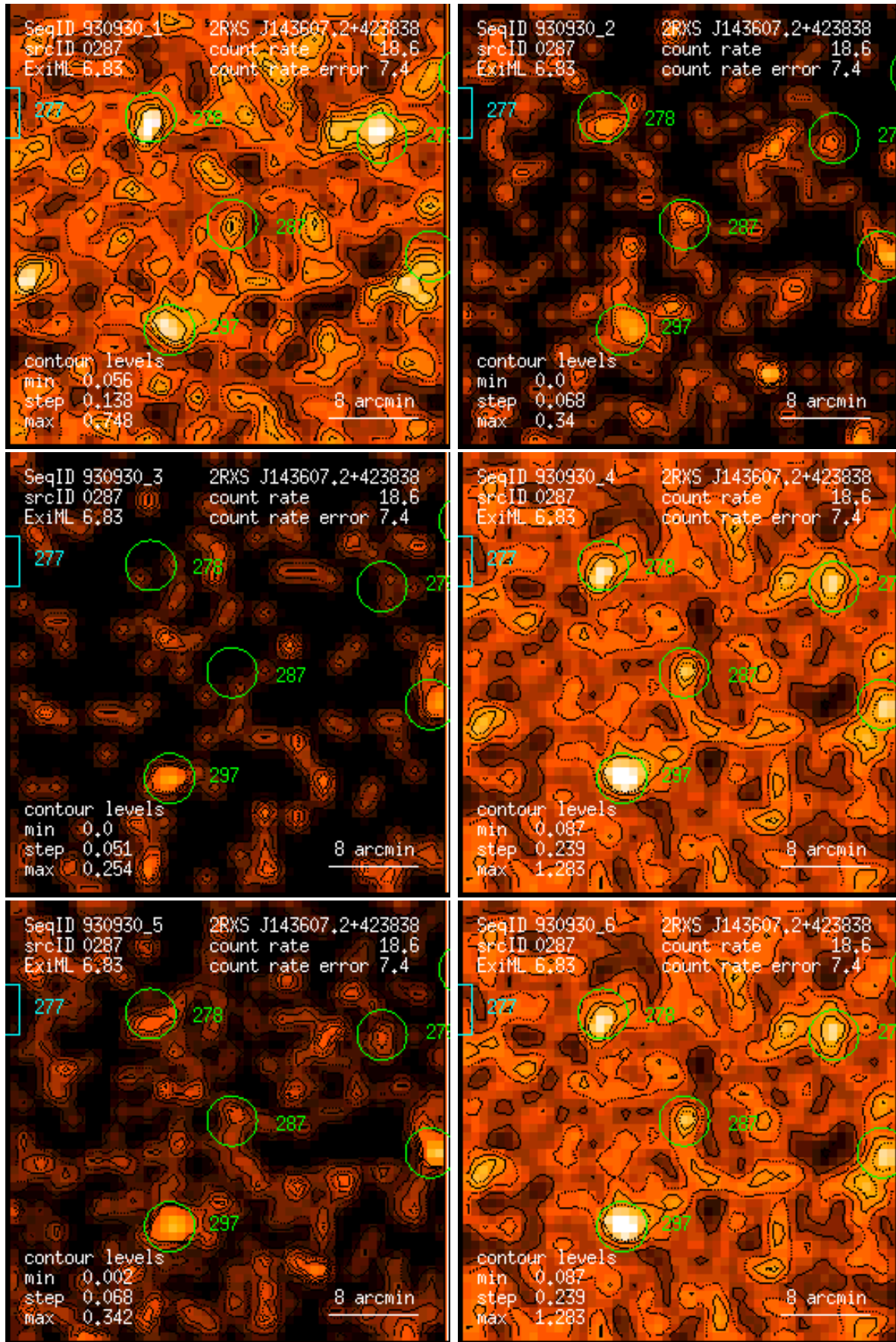
Figure 287: RASS 930930: detection 0287: band rate images, Gaussian filter: (1) PSPC channels 11 – 41, (2) 52 – 90, (3) 91 – 201, (4) 11 – 235, (5) 52 – 201, (6) 11 – 201. Broad band rates in counts/ks. Band rate contour levels in counts/ks/arcmin 2 .
