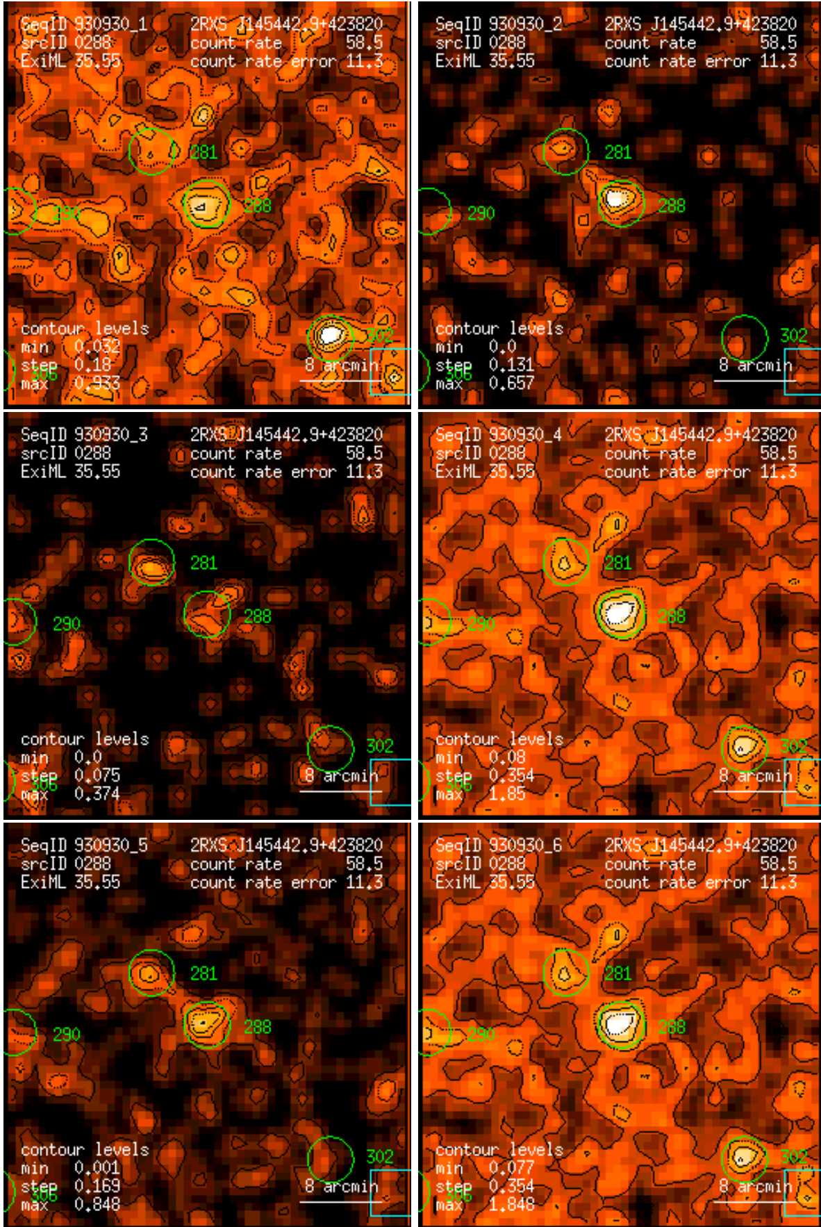
Figure 288: RASS 930930: detection 0288: band rate images, Gaussian filter: (1) PSPC channels 11 – 41, (2) 52 – 90, (3) 91 – 201, (4) 11 – 235, (5) 52 – 201, (6) 11 – 201. Broad band rates in counts/ks. Band rate contour levels in counts/ks/arcmin 2 .
