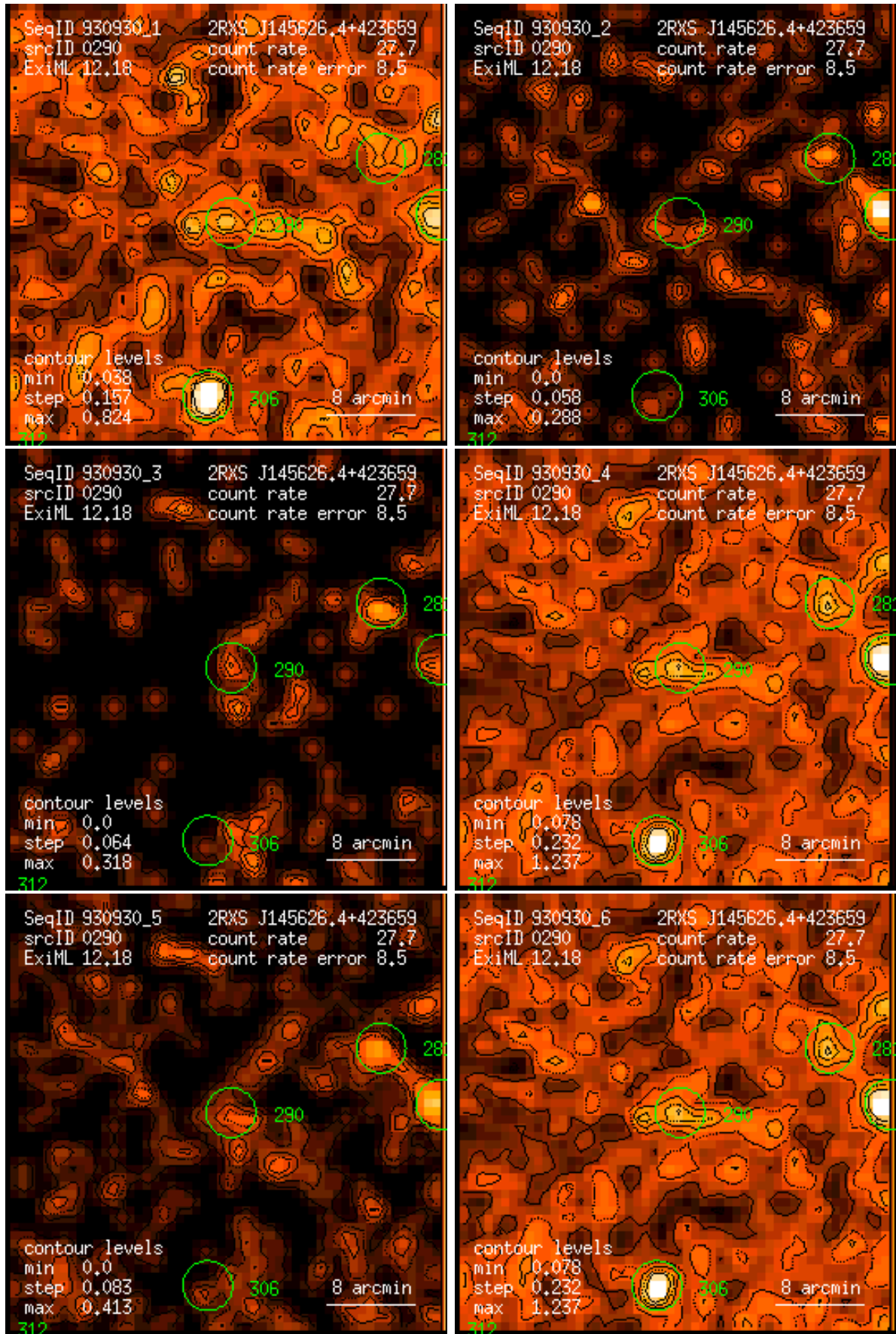
Figure 290: RASS 930930: detection 0290: band rate images, Gaussian filter: (1) PSPC channels 11 – 41, (2) 52 – 90, (3) 91 – 201, (4) 11 – 235, (5) 52 – 201, (6) 11 – 201. Broad band rates in counts/ks. Band rate contour levels in counts/ks/arcmin 2 .
