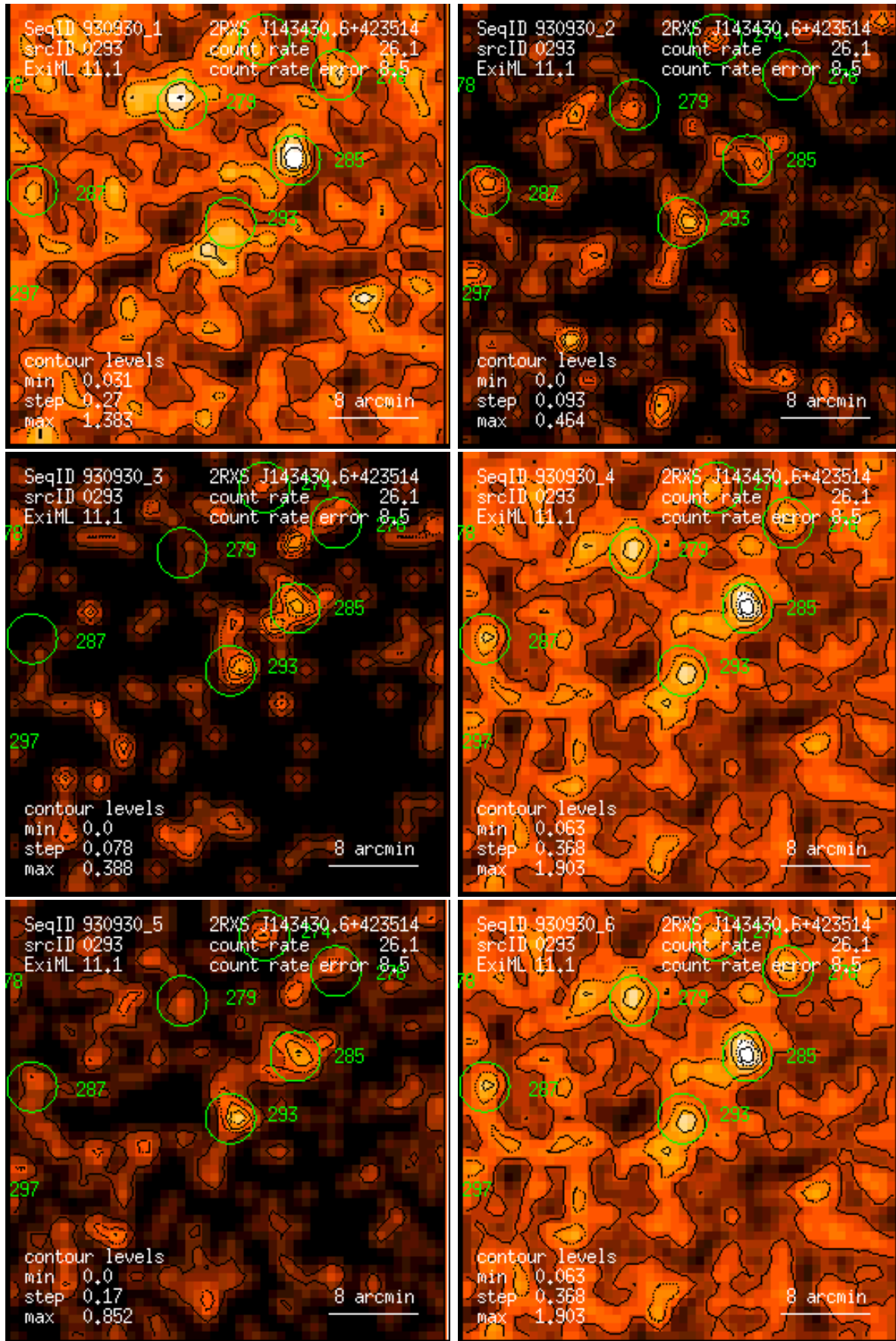
Figure 293: RASS 930930: detection 0293: band rate images, Gaussian filter: (1) PSPC channels 11 – 41, (2) 52 – 90, (3) 91 – 201, (4) 11 – 235, (5) 52 – 201, (6) 11 – 201. Broad band rates in counts/ks. Band rate contour levels in counts/ks/arcmin 2 .
