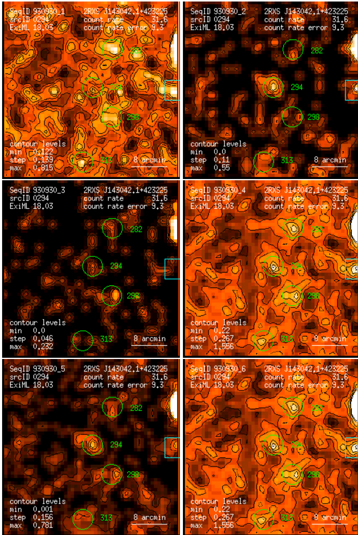
Figure 294: RASS 930930: detection 0294: band rate images, Gaussian filter: (1) PSPC channels 11 – 41, (2) 52 – 90, (3) 91 – 201, (4) 11 – 235, (5) 52 – 201, (6) 11 – 201. Broad band rates in counts/ks. Band rate contour levels in counts/ks/arcmin 2 .
