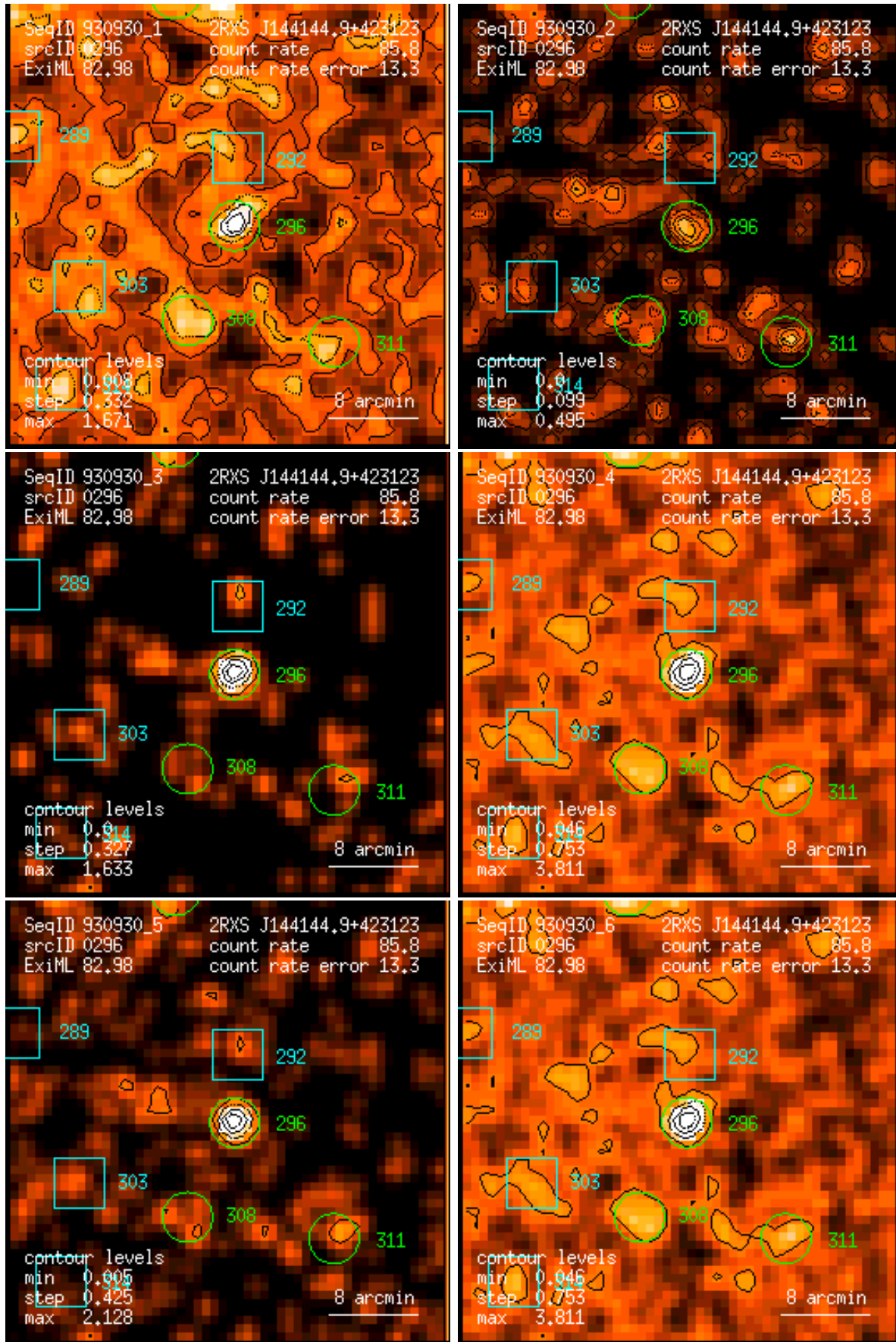
Figure 296: RASS 930930: detection 0296: band rate images, Gaussian filter: (1) PSPC channels 11 – 41, (2) 52 – 90, (3) 91 – 201, (4) 11 – 235, (5) 52 – 201, (6) 11 – 201. Broad band rates in counts/ks. Band rate contour levels in counts/ks/arcmin 2 .
