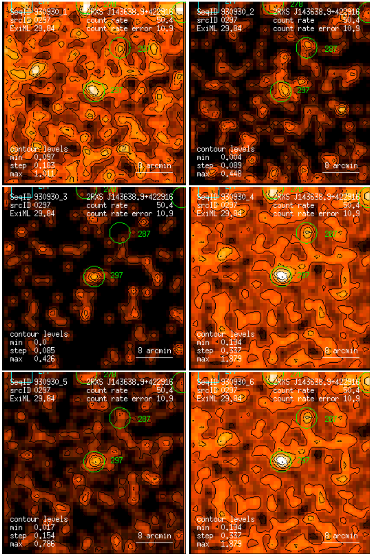
Figure 297: RASS 930930: detection 0297: band rate images, Gaussian filter: (1) PSPC channels 11 – 41, (2) 52 – 90, (3) 91 – 201, (4) 11 – 235, (5) 52 – 201, (6) 11 – 201. Broad band rates in counts/ks. Band rate contour levels in counts/ks/arcmin 2 .
