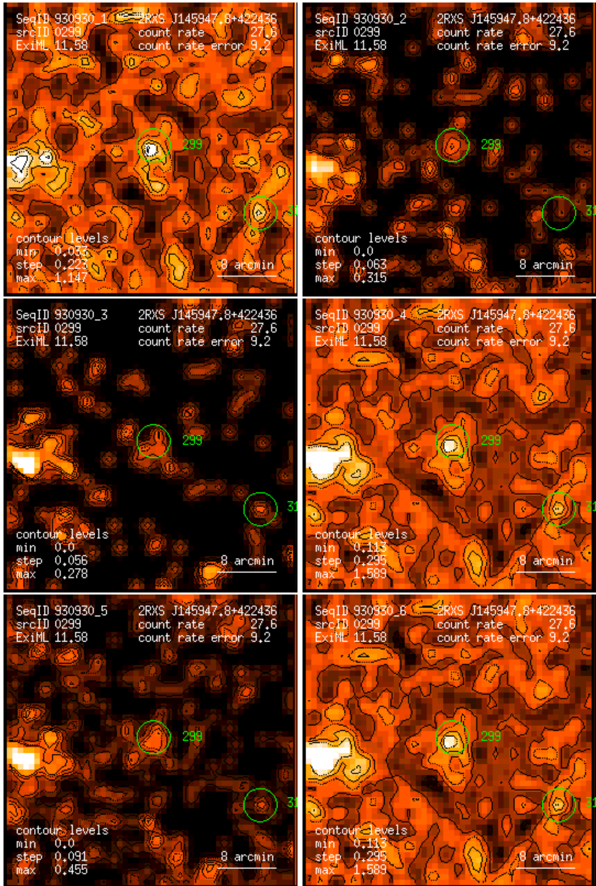
Figure 299: RASS 930930: detection 0299: band rate images, Gaussian filter: (1) PSPC channels 11 – 41, (2) 52 – 90, (3) 91 – 201, (4) 11 – 235, (5) 52 – 201, (6) 11 – 201. Broad band rates in counts/ks. Band rate contour levels in counts/ks/arcmin 2 .
