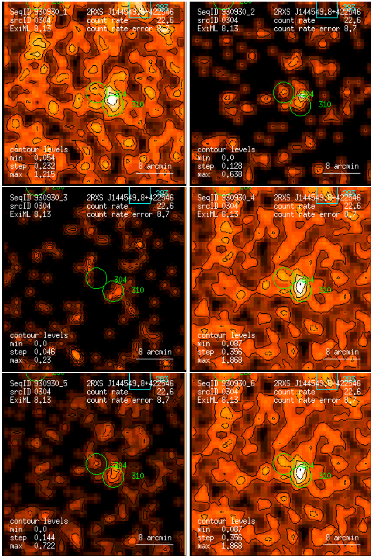
Figure 304: RASS 930930: detection 0304: band rate images, Gaussian filter: (1) PSPC channels 11 – 41, (2) 52 – 90, (3) 91 – 201, (4) 11 – 235, (5) 52 – 201, (6) 11 – 201. Broad band rates in counts/ks. Band rate contour levels in counts/ks/arcmin 2 .
