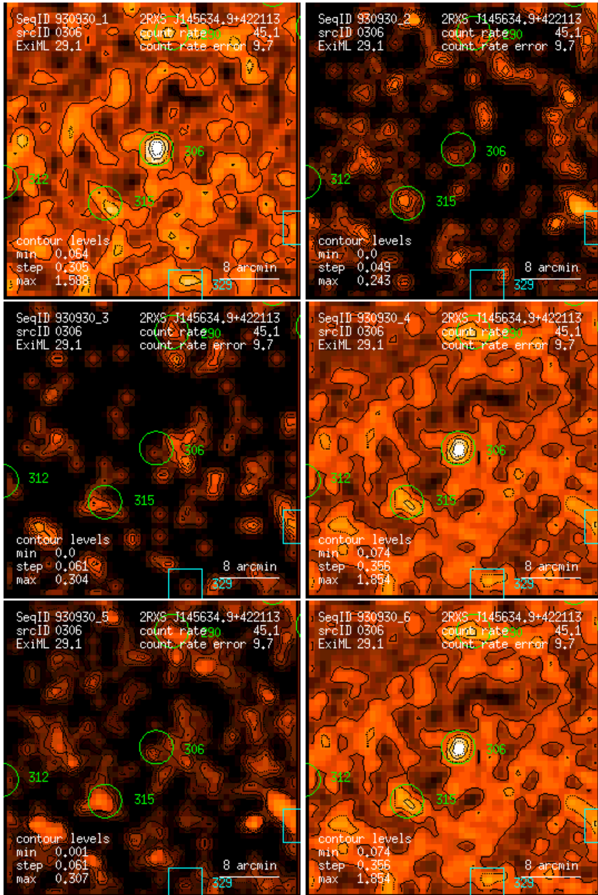
Figure 306: RASS 930930: detection 0306: band rate images, Gaussian filter: (1) PSPC channels 11 – 41, (2) 52 – 90, (3) 91 – 201, (4) 11 – 235, (5) 52 – 201, (6) 11 – 201. Broad band rates in counts/ks. Band rate contour levels in counts/ks/arcmin 2 .
