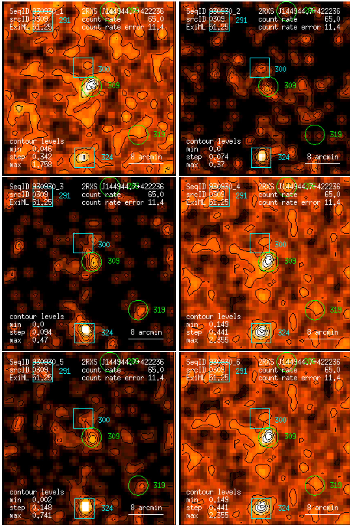
Figure 309: RASS 930930: detection 0309: band rate images, Gaussian filter: (1) PSPC channels 11 – 41, (2) 52 – 90, (3) 91 – 201, (4) 11 – 235, (5) 52 – 201, (6) 11 – 201. Broad band rates in counts/ks. Band rate contour levels in counts/ks/arcmin 2 .
