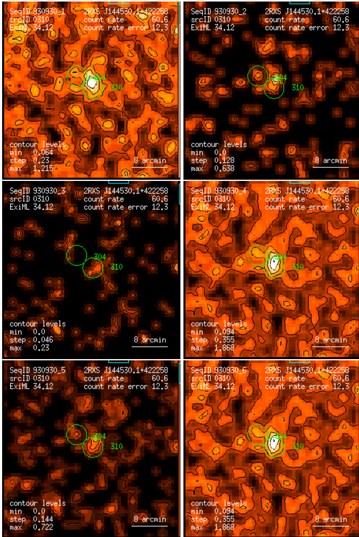
Figure 310: RASS 930930: detection 0310: band rate images, Gaussian filter: (1) PSPC channels 11 – 41, (2) 52 – 90, (3) 91 – 201, (4) 11 – 235, (5) 52 – 201, (6) 11 – 201. Broad band rates in counts/ks. Band rate contour levels in counts/ks/arcmin 2 .
