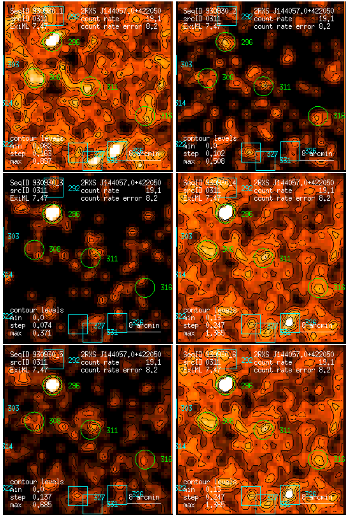
Figure 311: RASS 930930: detection 0311: band rate images, Gaussian filter: (1) PSPC channels 11 – 41, (2) 52 – 90, (3) 91 – 201, (4) 11 – 235, (5) 52 – 201, (6) 11 – 201. Broad band rates in counts/ks. Band rate contour levels in counts/ks/arcmin 2 .
