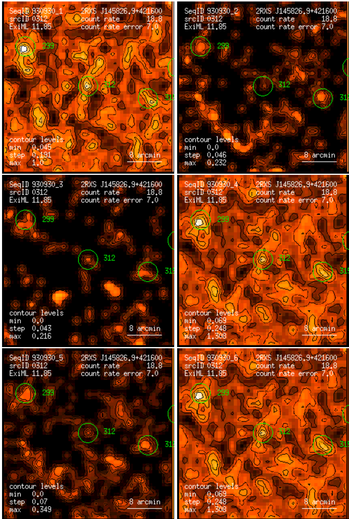
Figure 312: RASS 930930: detection 0312: band rate images, Gaussian filter: (1) PSPC channels 11 – 41, (2) 52 – 90, (3) 91 – 201, (4) 11 – 235, (5) 52 – 201, (6) 11 – 201. Broad band rates in counts/ks. Band rate contour levels in counts/ks/arcmin 2 .
