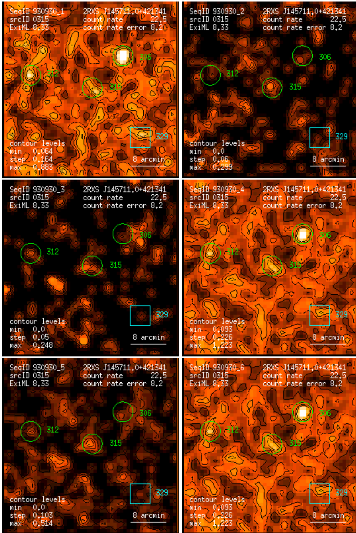
Figure 315: RASS 930930: detection 0315: band rate images, Gaussian filter: (1) PSPC channels 11 – 41, (2) 52 – 90, (3) 91 – 201, (4) 11 – 235, (5) 52 – 201, (6) 11 – 201. Broad band rates in counts/ks. Band rate contour levels in counts/ks/arcmin 2 .
