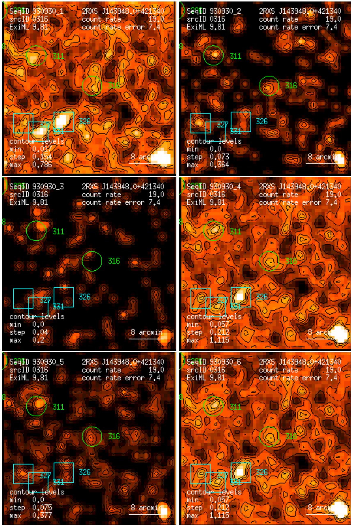
Figure 316: RASS 930930: detection 0316: band rate images, Gaussian filter: (1) PSPC channels 11 – 41, (2) 52 – 90, (3) 91 – 201, (4) 11 – 235, (5) 52 – 201, (6) 11 – 201. Broad band rates in counts/ks. Band rate contour levels in counts/ks/arcmin 2 .
