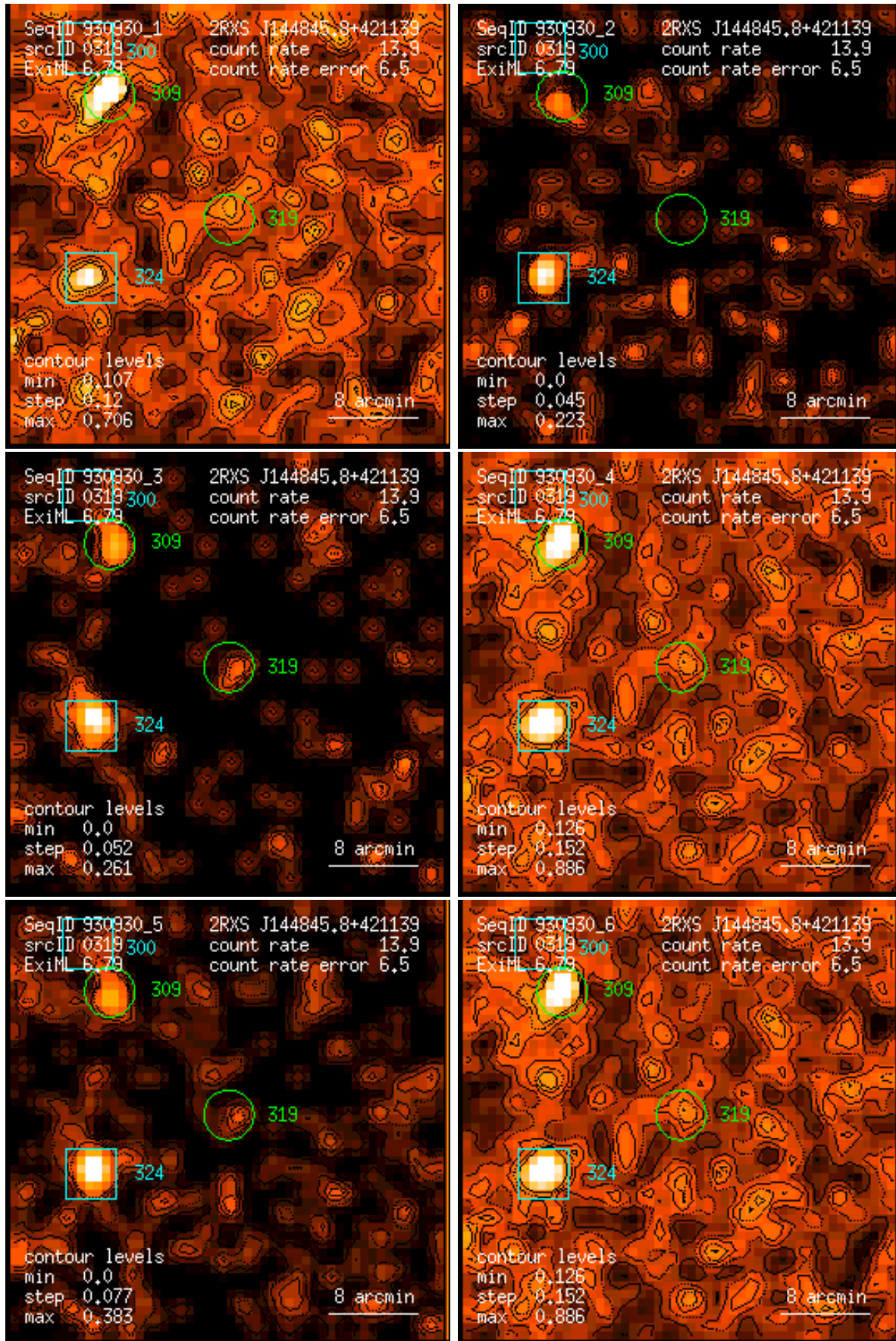
Figure 319: RASS 930930: detection 0319: band rate images, Gaussian filter: (1) PSPC channels 11 – 41, (2) 52 – 90, (3) 91 – 201, (4) 11 – 235, (5) 52 – 201, (6) 11 – 201. Broad band rates in counts/ks. Band rate contour levels in counts/ks/arcmin 2 .
