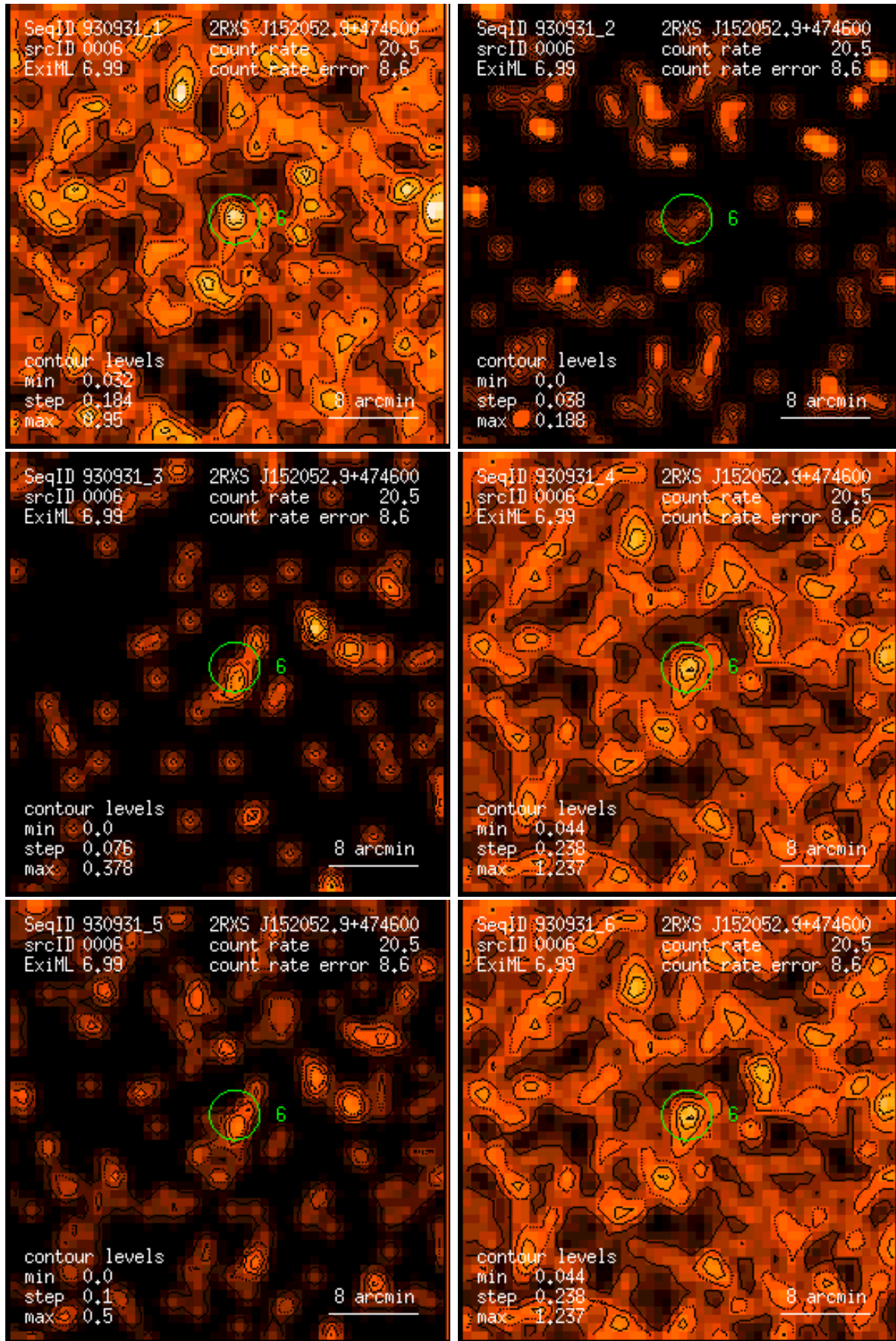
Figure 6: RASS 930931: detection 0006: band rate images, Gaussian filter: (1) PSPC channels 11 – 41, (2) 52 – 90, (3) 91 – 201, (4) 11 – 235, (5) 52 – 201, (6) 11 – 201. Broad band rates in counts/ks. Band rate contour levels in counts/ks/arcmin 2 .
