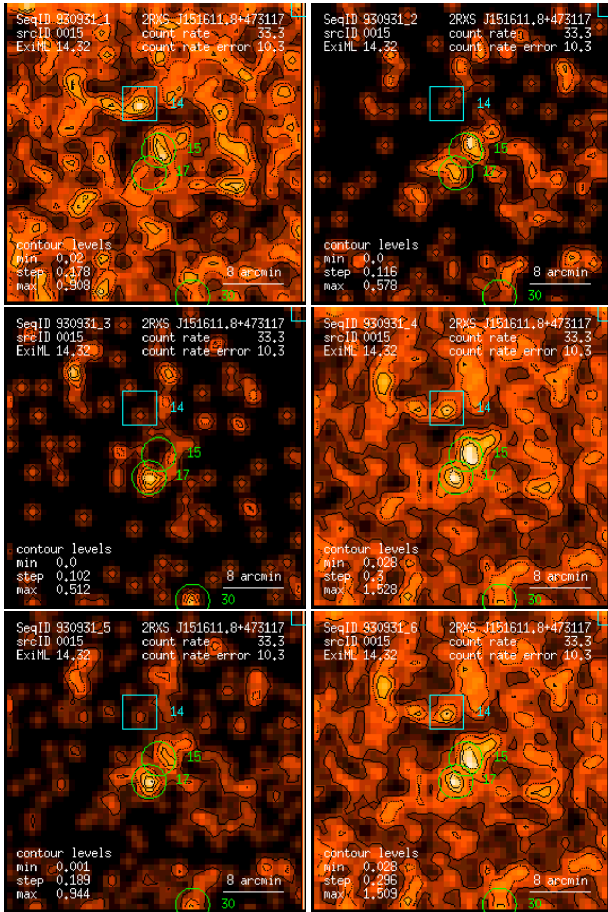
Figure 15: RASS 930931: detection 0015: band rate images, Gaussian filter: (1) PSPC channels 11 – 41, (2) 52 – 90, (3) 91 – 201, (4) 11 – 235, (5) 52 – 201, (6) 11 – 201. Broad band rates in counts/ks. Band rate contour levels in counts/ks/arcmin 2 .
