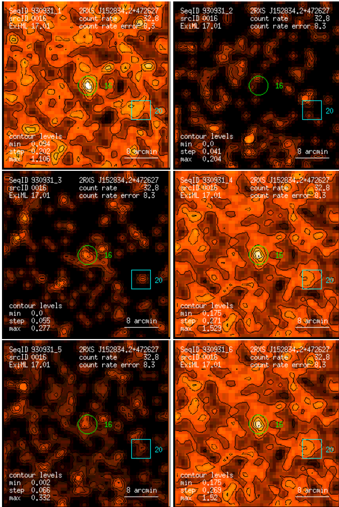
Figure 16: RASS 930931: detection 0016: band rate images, Gaussian filter: (1) PSPC channels 11 – 41, (2) 52 – 90, (3) 91 – 201, (4) 11 – 235, (5) 52 – 201, (6) 11 – 201. Broad band rates in counts/ks. Band rate contour levels in counts/ks/arcmin 2 .
